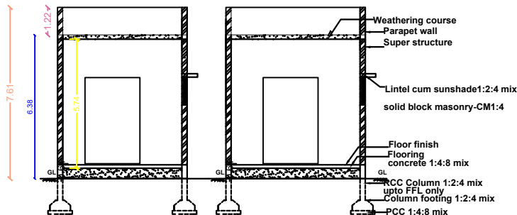
SECTION ELEVATION
