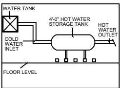
WATER TANK
