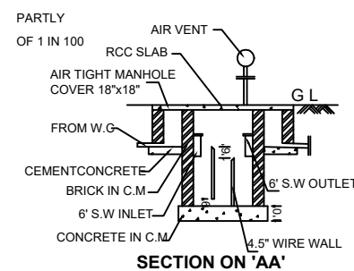
INSPECTION CHAMBER SEPTIC TANK DETAIL SCALE: NTS
