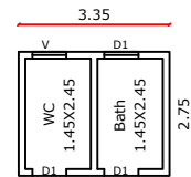
R TOILET BLOCK PLAN
