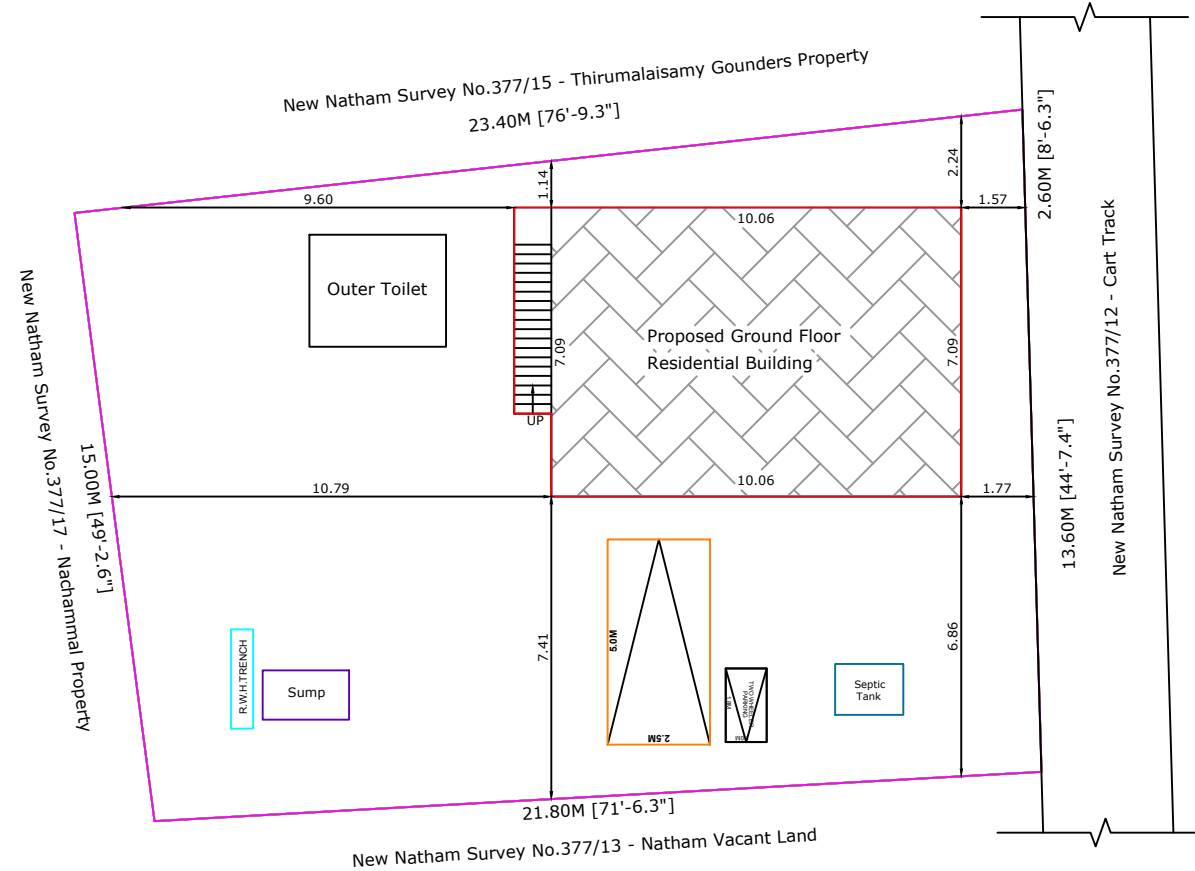
SITE PLAN
