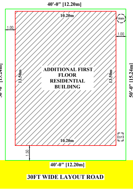
SITE PLAN
