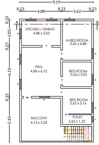
PRO.S.FLOOR PLAN
