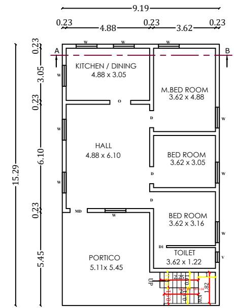
PRO.ADDL. & ALTERATION OF G.FLOOR PLAN
