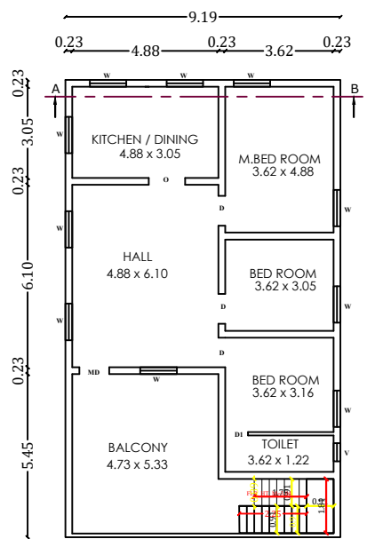
PRO.F.FLOOR PLAN
