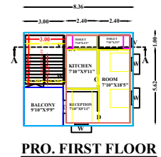
PRO. FIRST FLOOR
