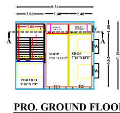
PRO. GROUND FLOOR
