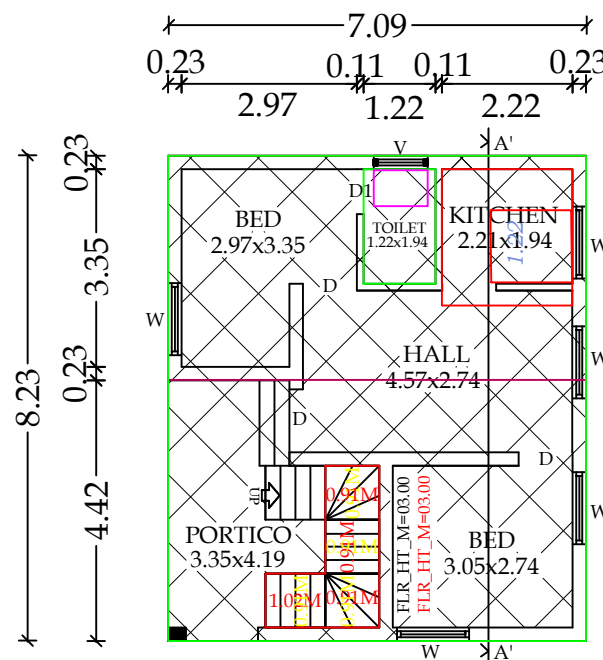
EXG. GROUND FLOOR PLAN
