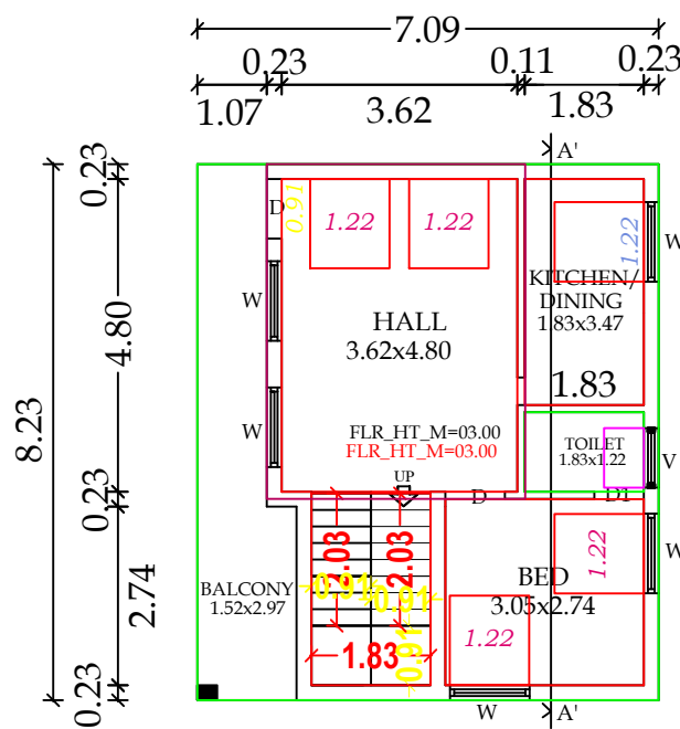
PRO.ADD. FIRST FLOOR PLAN
