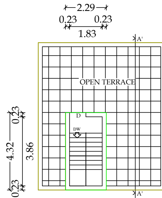
PRO. ADD. TERRACE FLOOR PLAN
