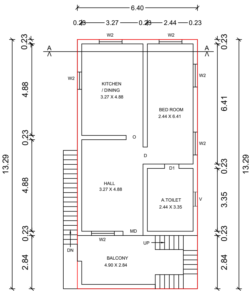
PROPOSED ADDITIONAL FIRST FLOOR PLAN (SCALE 1" EQ 8'-0")
