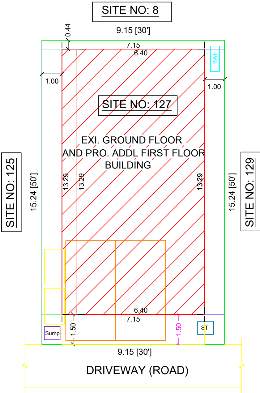
SITE PLAN (SCALE 1" EQ 8'-0")
