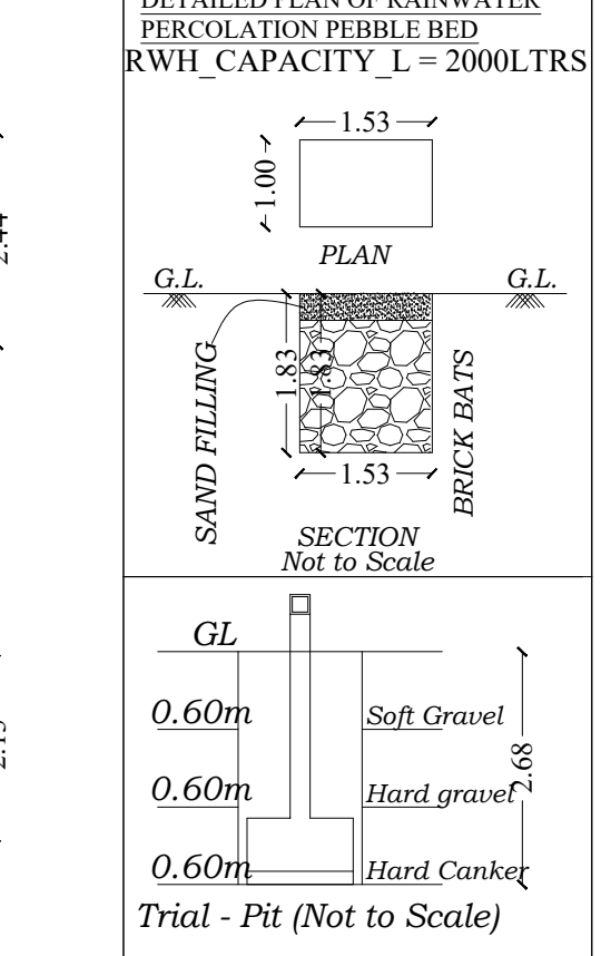
0.60m Hard Canker Trial - Pit (Not to Scale)
