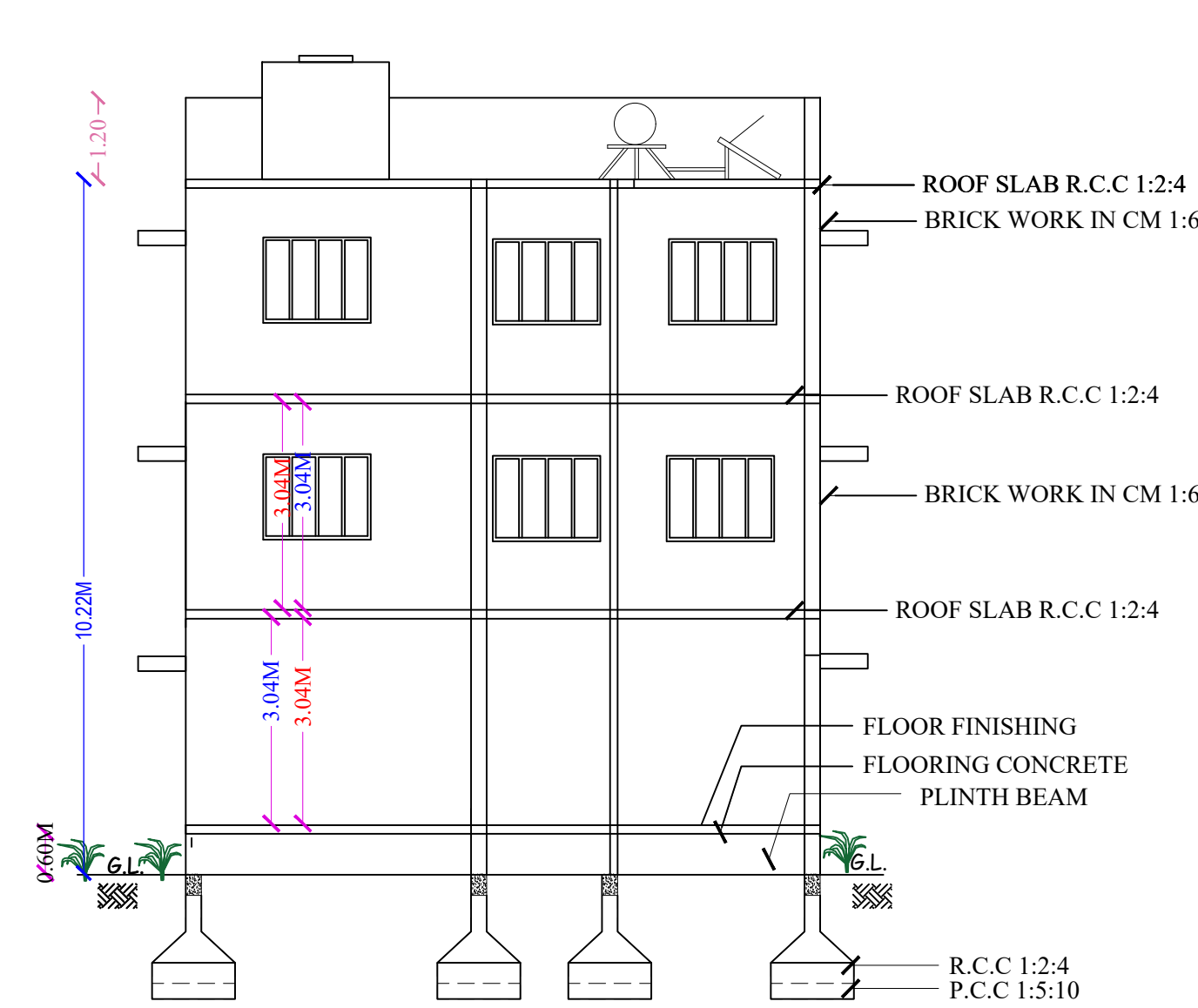
SECTION "A-A"
