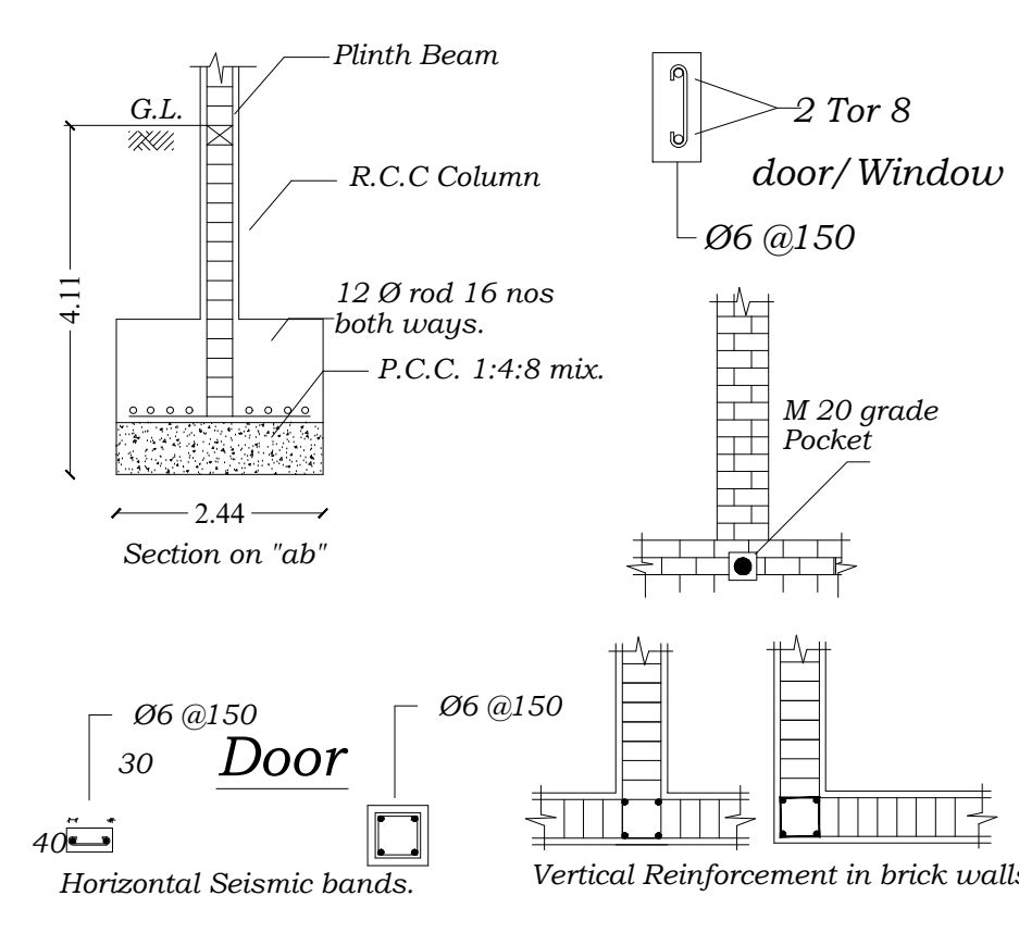
Horizontal Seismic bands. Vertical Reinforcement in brick wall.
