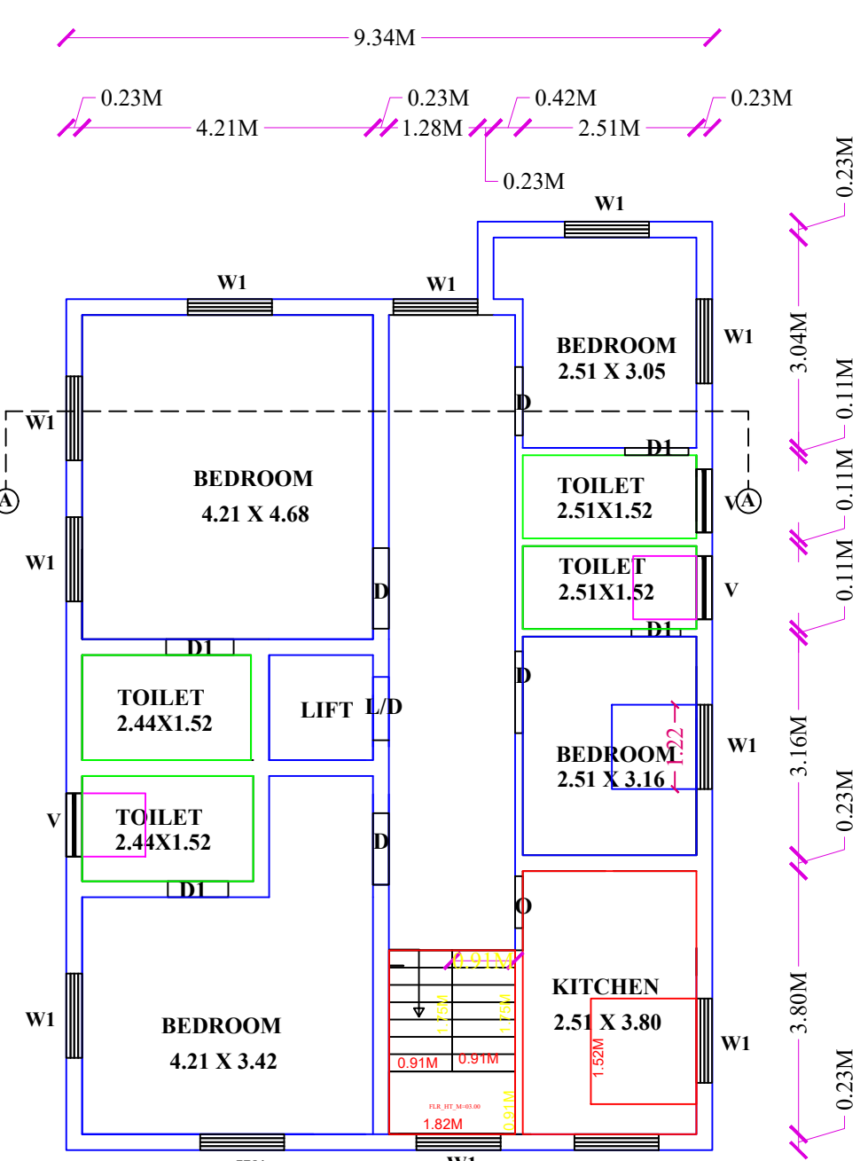
9.34M SECOND FLOOR
