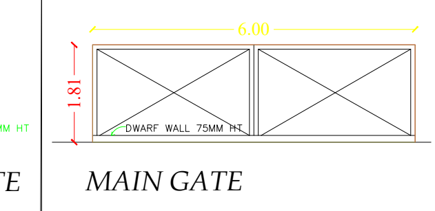
MAIN GATE
