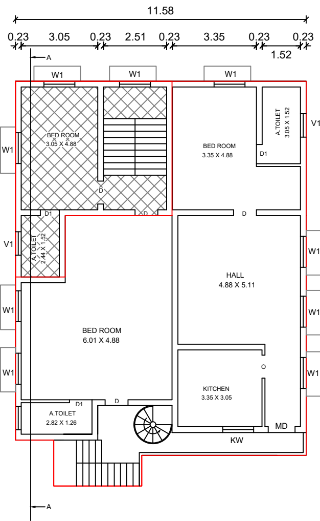
EXI & PRO FIRST FLOOR PLAN (SCALE 1" EQ 8'-0")
