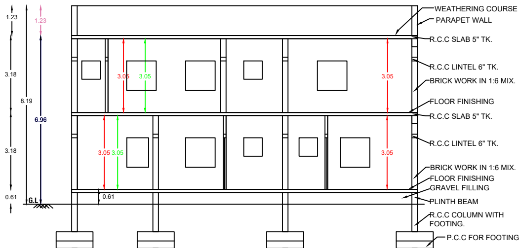
SECTION ON "AA" (SCALE 1" EQ 8'-0")
