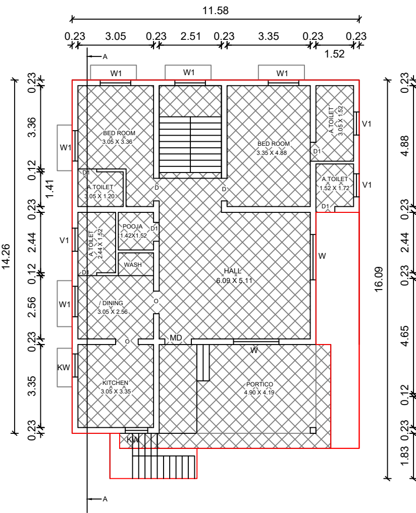
EXI & PRO GROUND FLOOR PLAN
