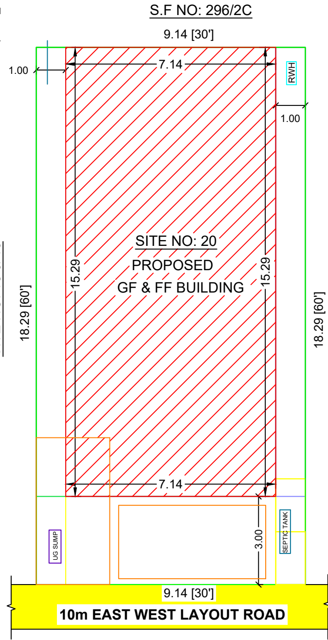
SITE PLAN
