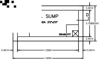
SUMP DETAIL SCALE 1"=4'0"
