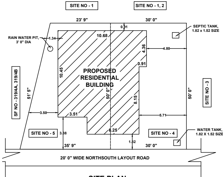
SITE PLAN SCALE - 1" 0" = 10' 0"
