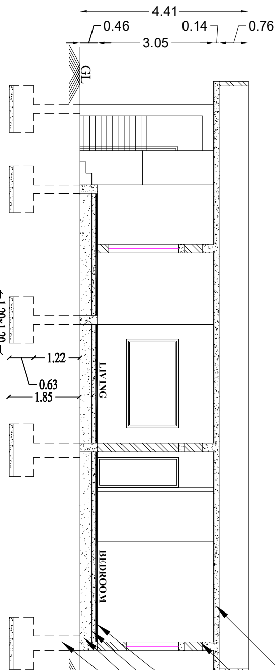
SECTION ON AA
