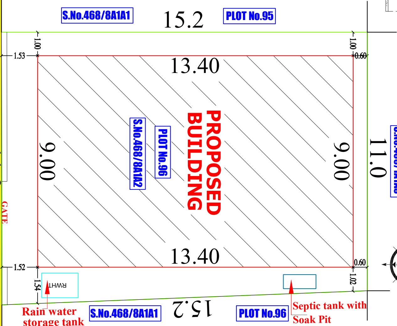
SITE PLAN
