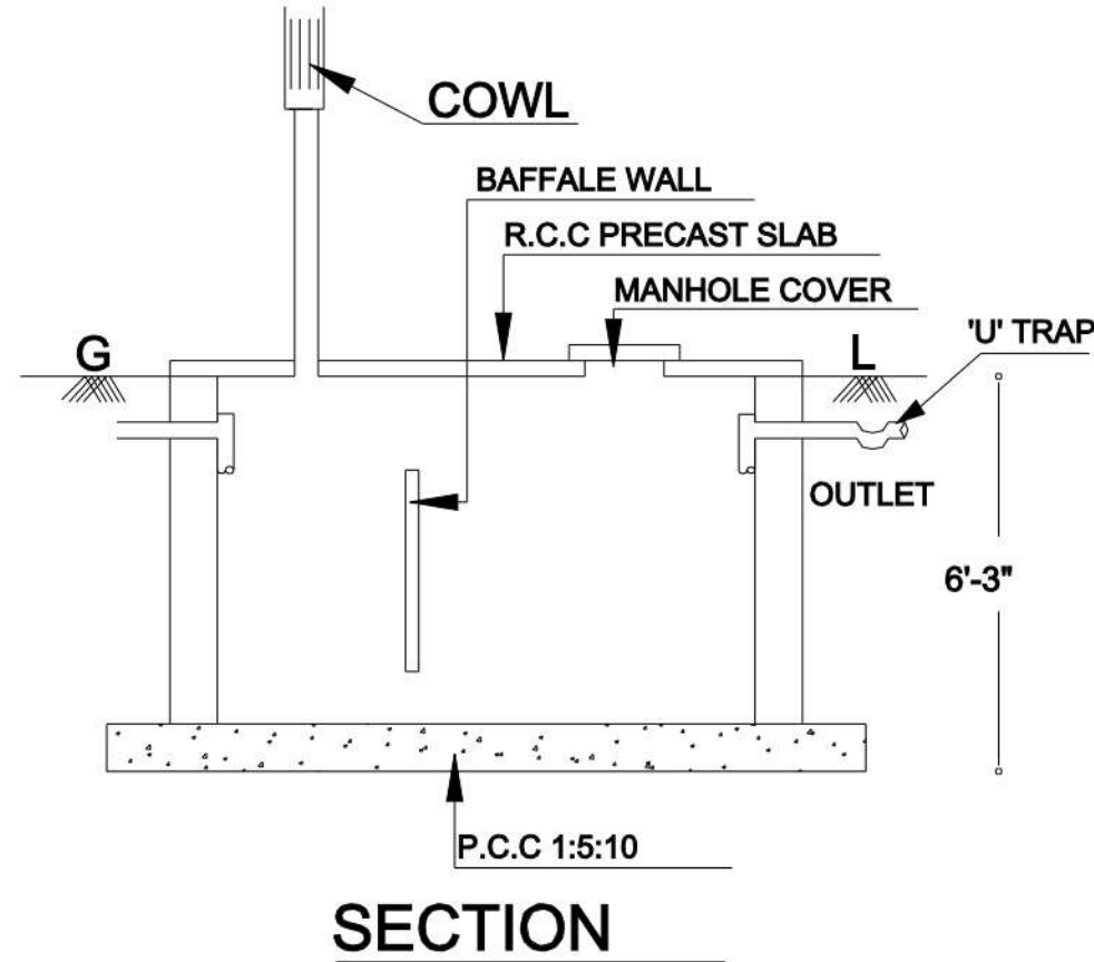
SECTION
