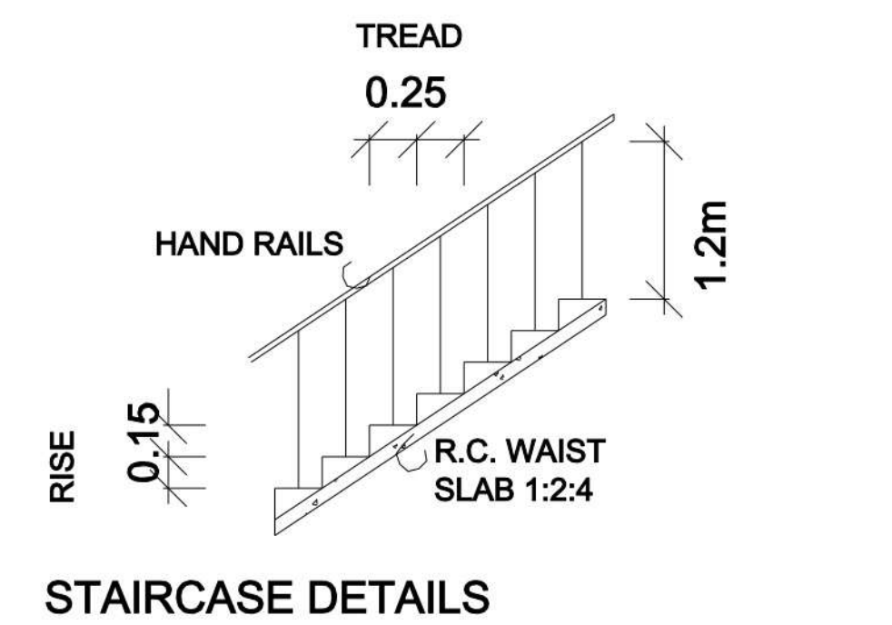
STAIRCASE DETAILS
