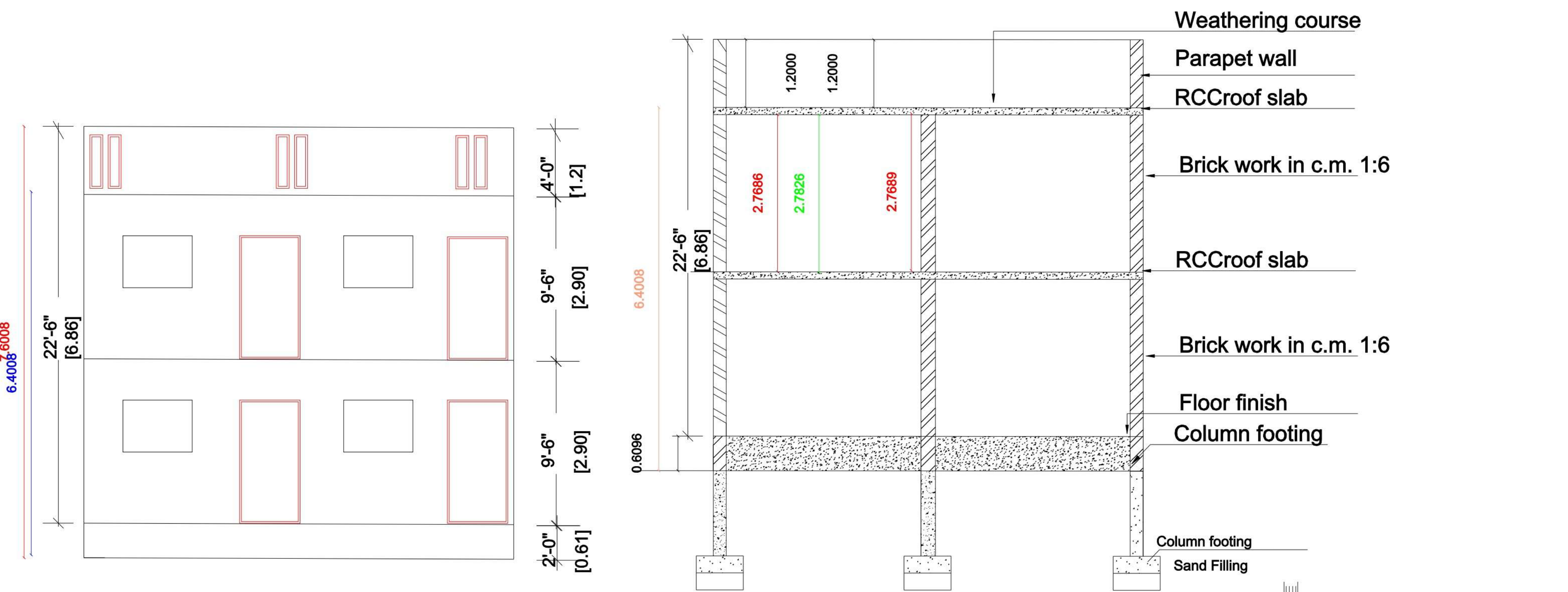
FRONT ELEVATION
