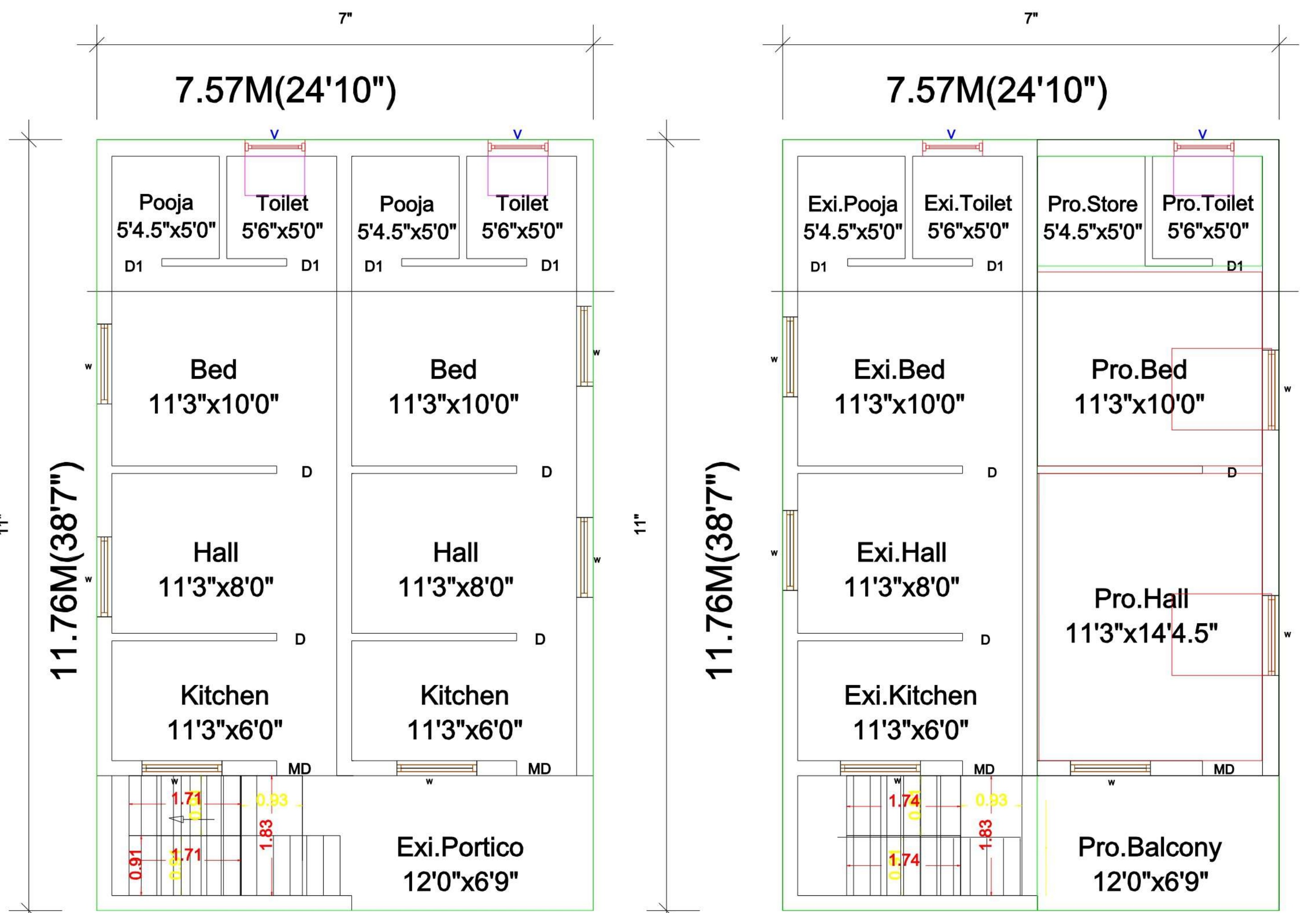
EXI.GROUND FLOOR PLAN
