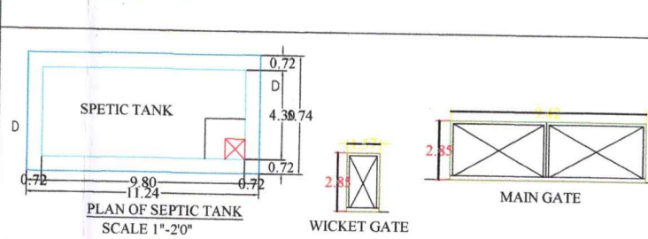
DETAILED DRAWING FOR SEPTIC TANK WITH DISPERSION TRENCH 225 GALLONS CAPACITY OF 1000 LITRES MANHOLE 0.45 SQW WITH AIR TIGHT COVER VENTILATOR SHAFT 0.10 DIA SW PIPE OPEN JOINT AND LAID TO A FALL OF 1/100 FORMATION LEVEL COUNTRY ROOF PAN TILES EXTRA LARGE TO COVER SIDES PARTIALLY 0.15 OSW INLET 0.15 OSW OUTLET BRICK WORK IN CM 1:3 SECTION OF SEPTIC TANK INSPECTION CHAMBER 0.3 TK SAND ENCLOSING ALL SIDES PLAN OF SEPTIC TANK PLAN OF DISPERSION TRENCH
