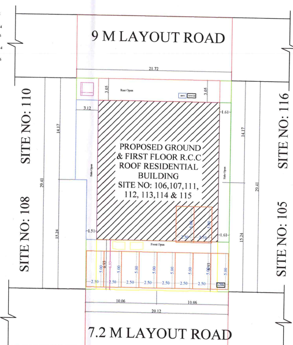
SITE PLAN
