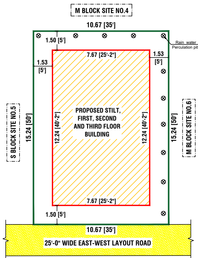
SITE PLAN
