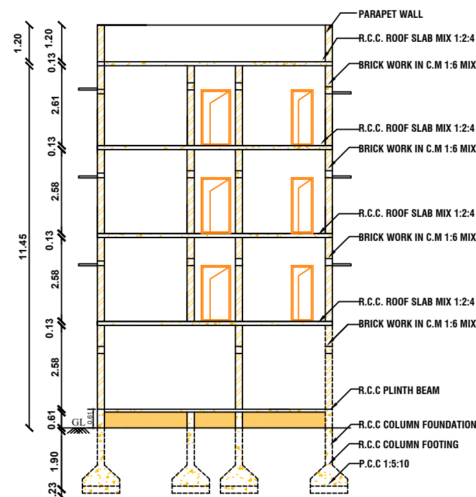
CROSS SECTION AT A-A
