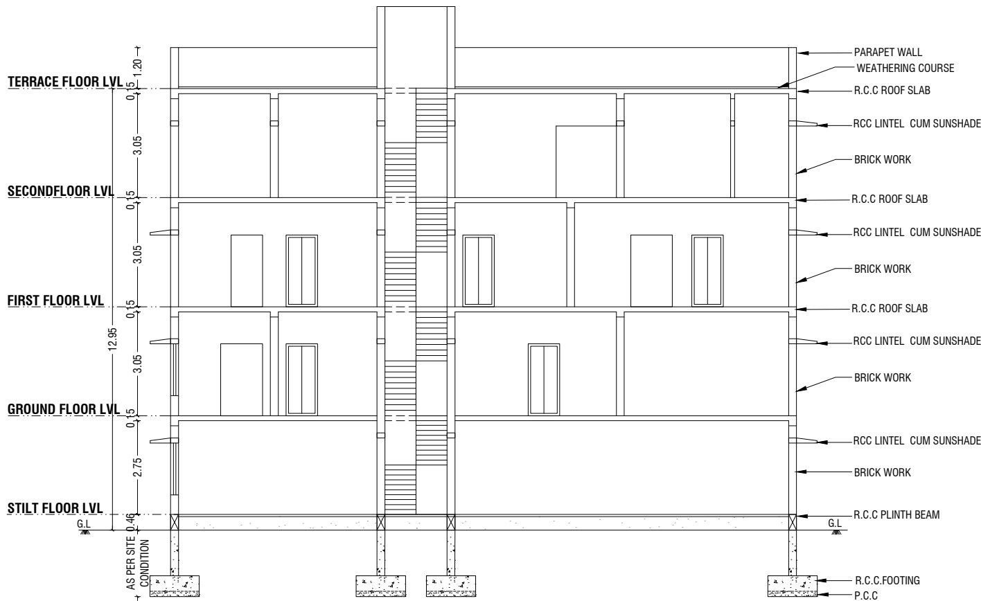
SECTION "AA" @ SOUTH SIDE
