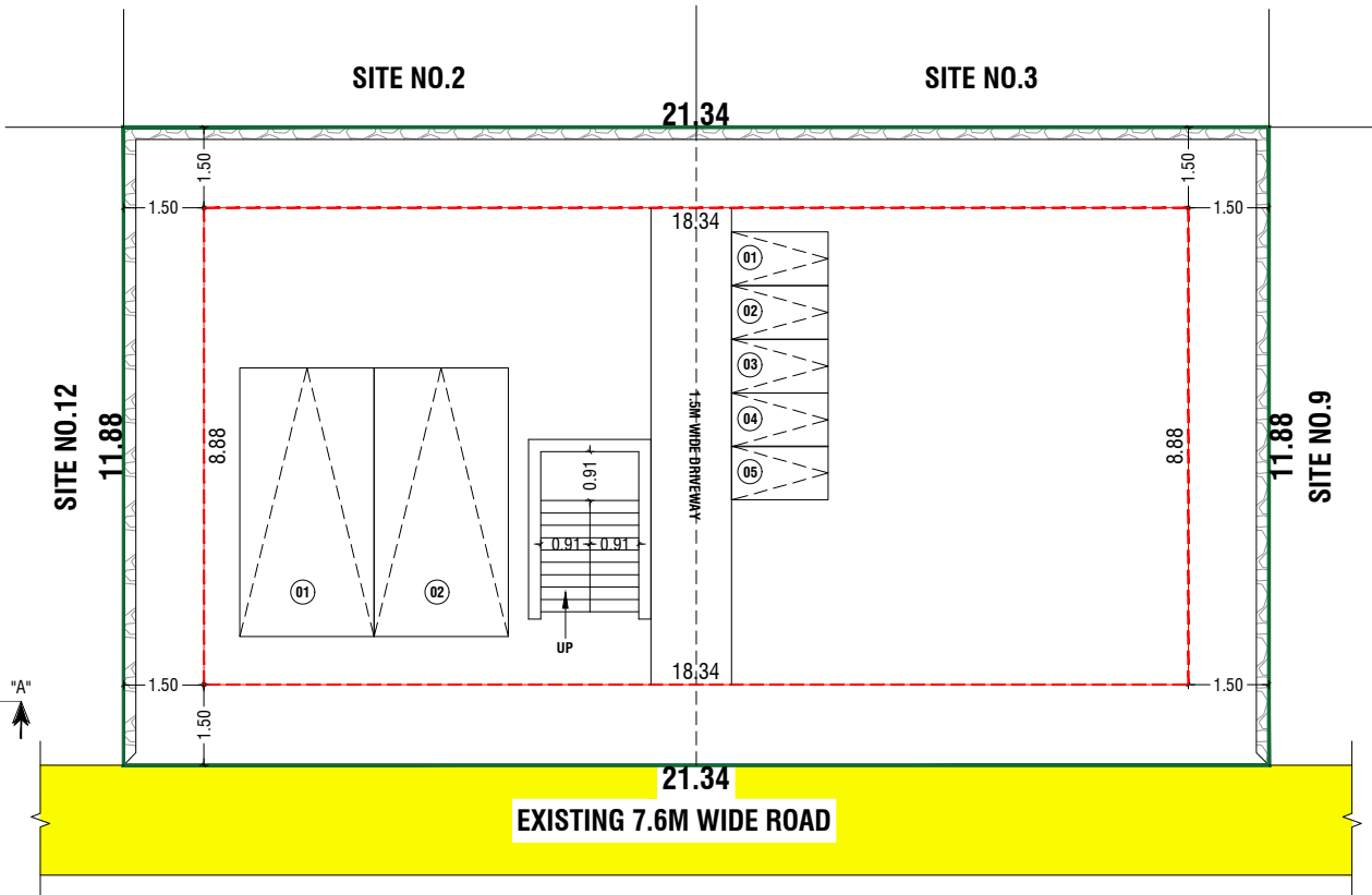
SITE CUM STILT FLOOR PLAN
