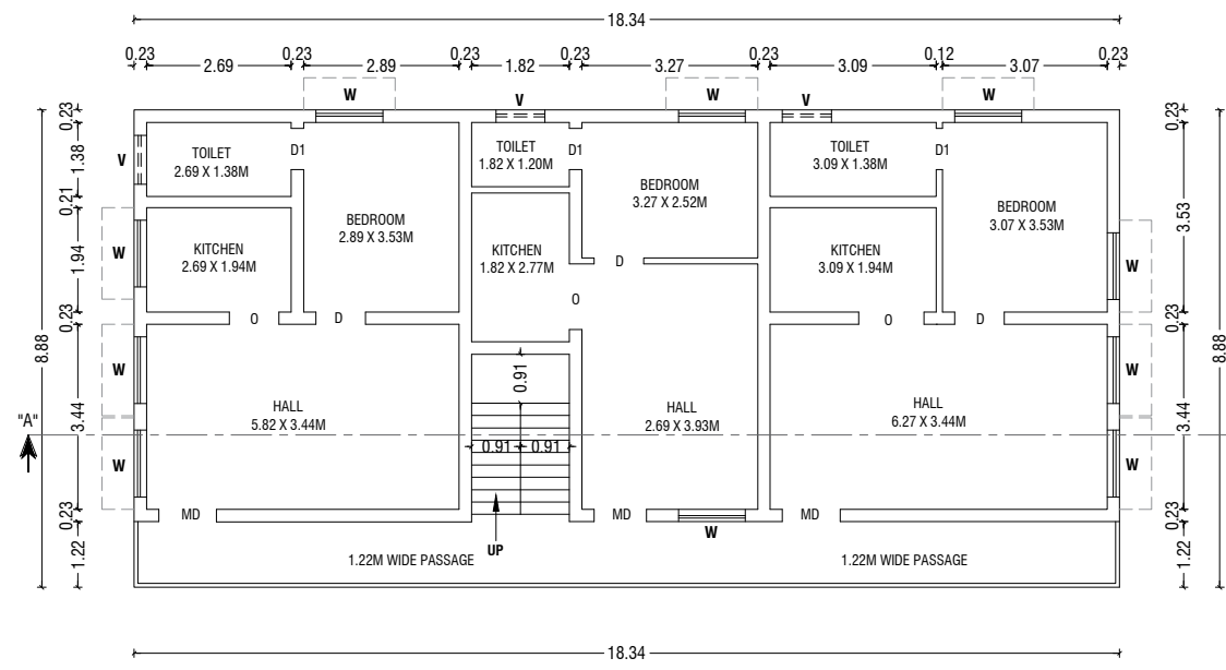
SECOND FLOOR
