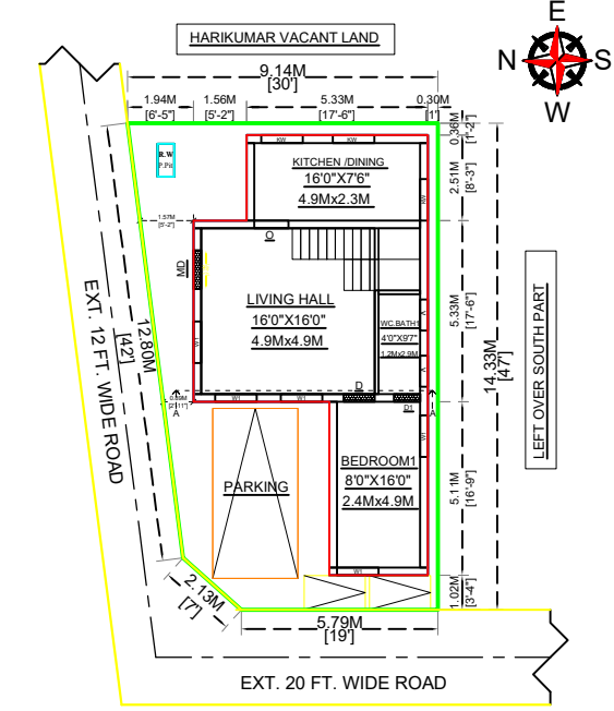
Site cum Proposed Ground Floor Plan
