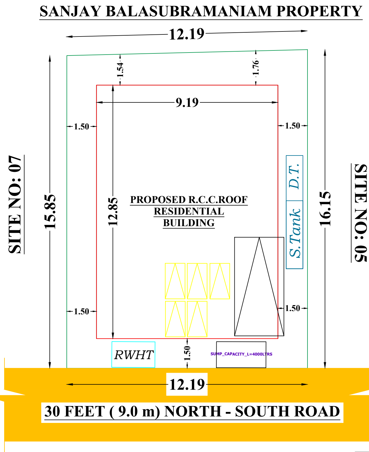
SITE PLAN
