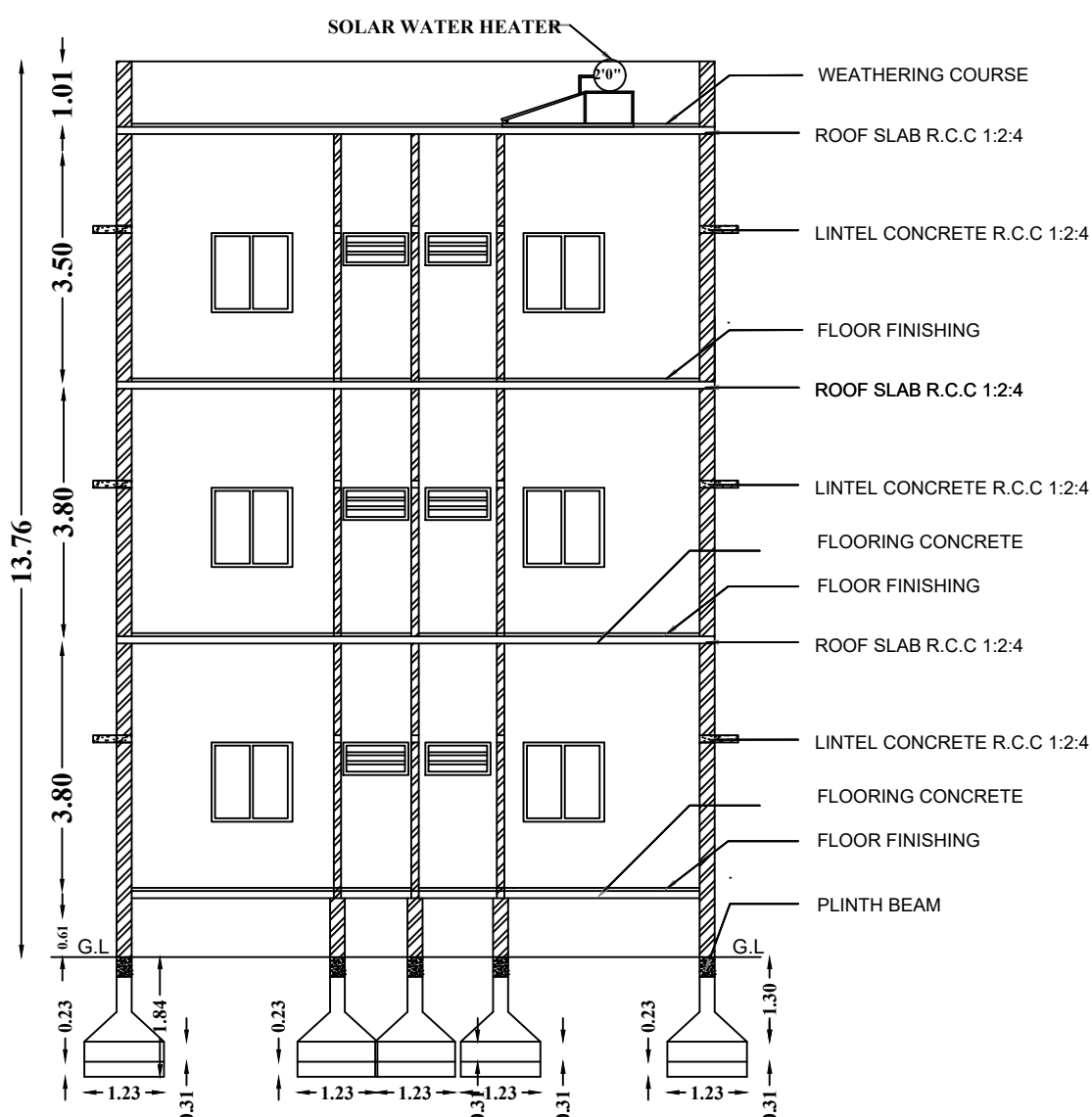
SECTION
