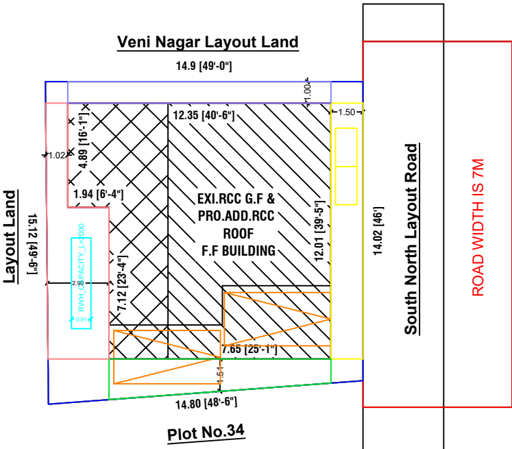
SITE PLAN
