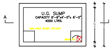
SUMP DETAIL
