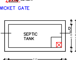
PLAN OF SEPTIC TANK
