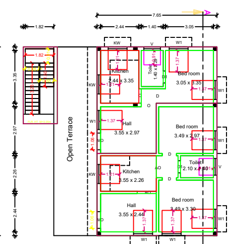
PRO.ADD. FIRST FLOOR
