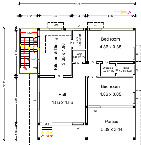
EXI. GROUND FLOOR
