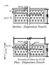
Plan - Dispersion Trench
