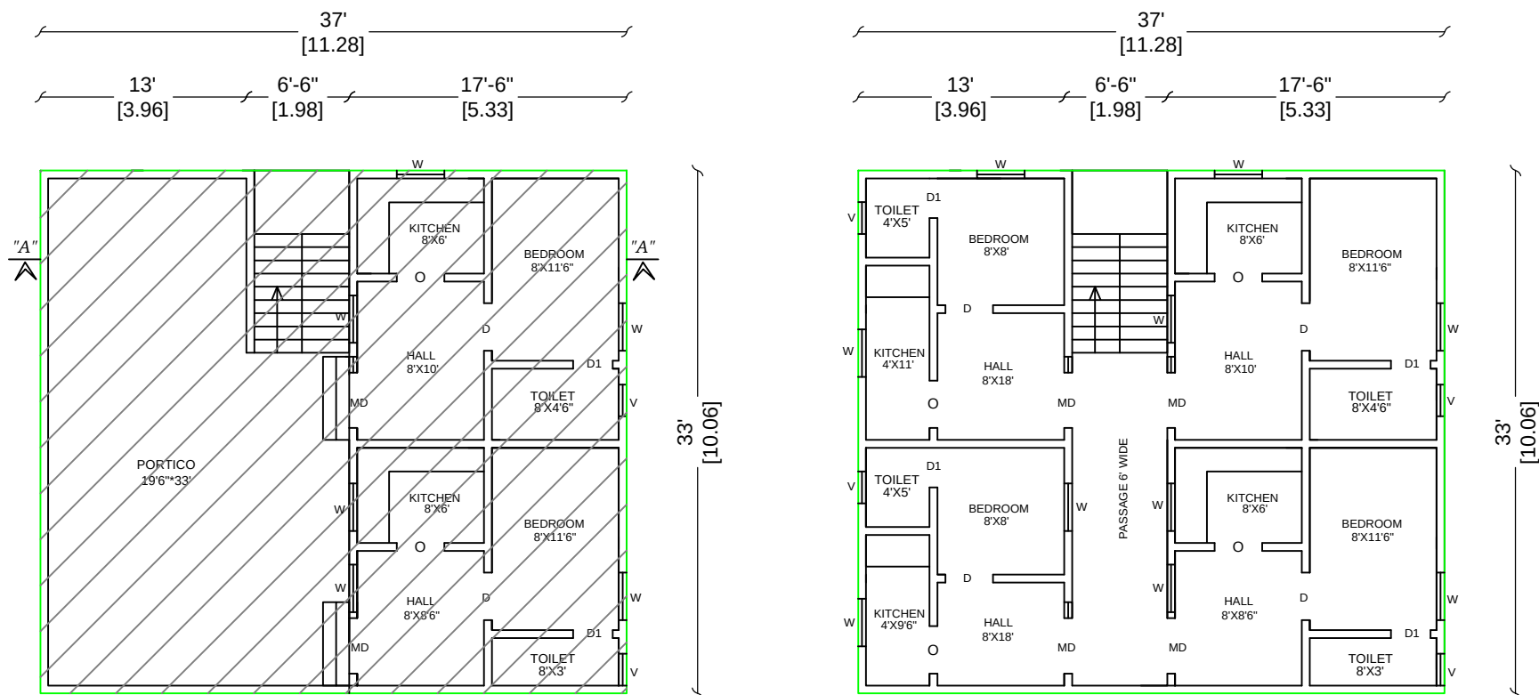
EXIS. GROUND FLOOR PLAN
