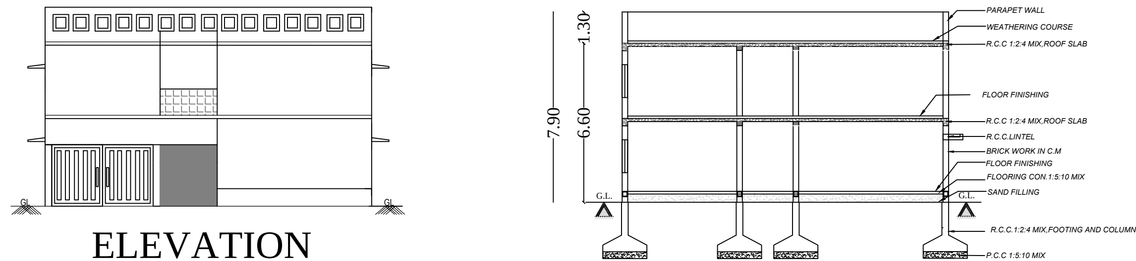
SECTION "A-A"
