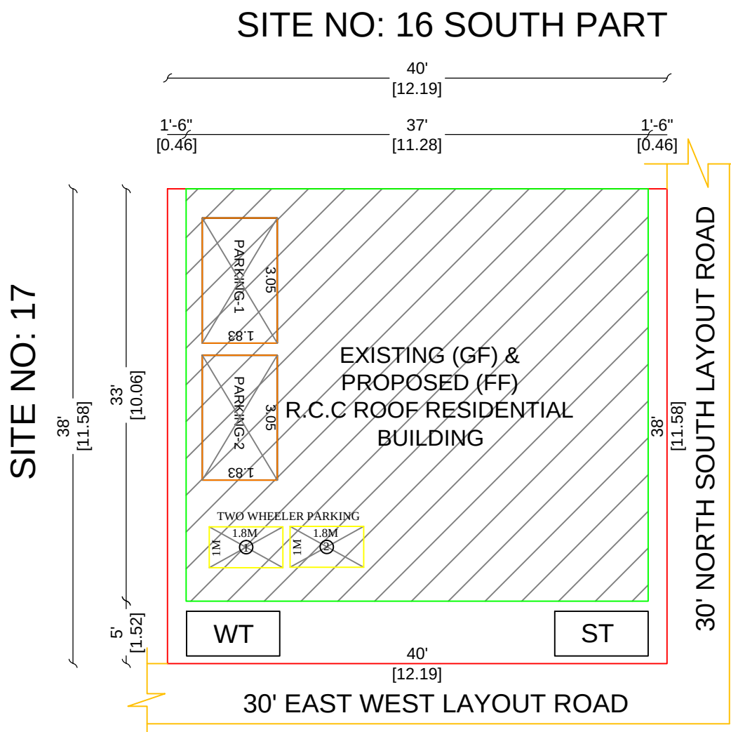
SITE PLAN
