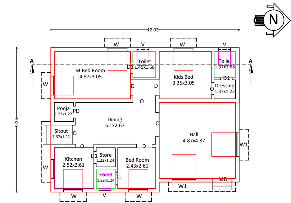
GF PLAN
