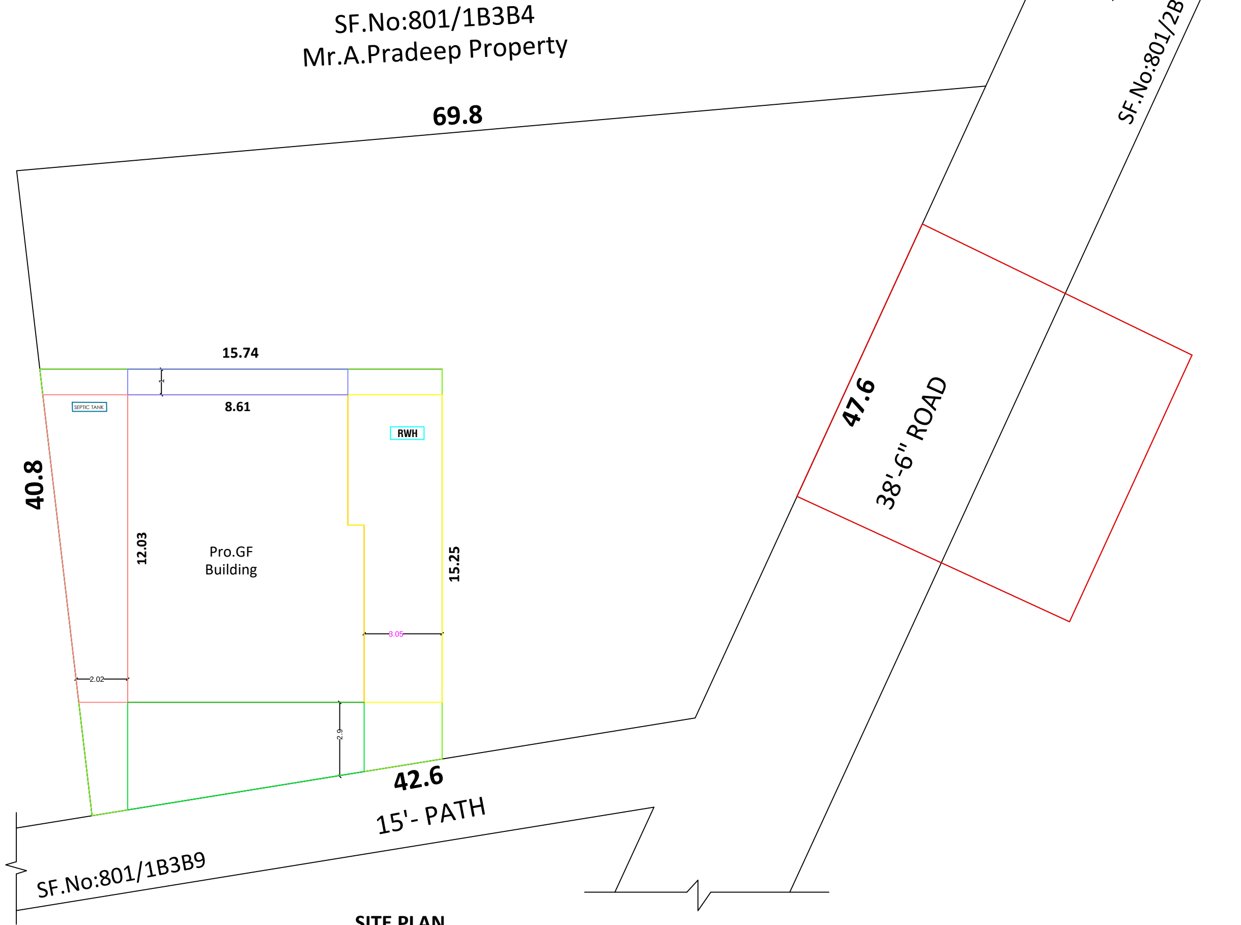
SITE PLAN
