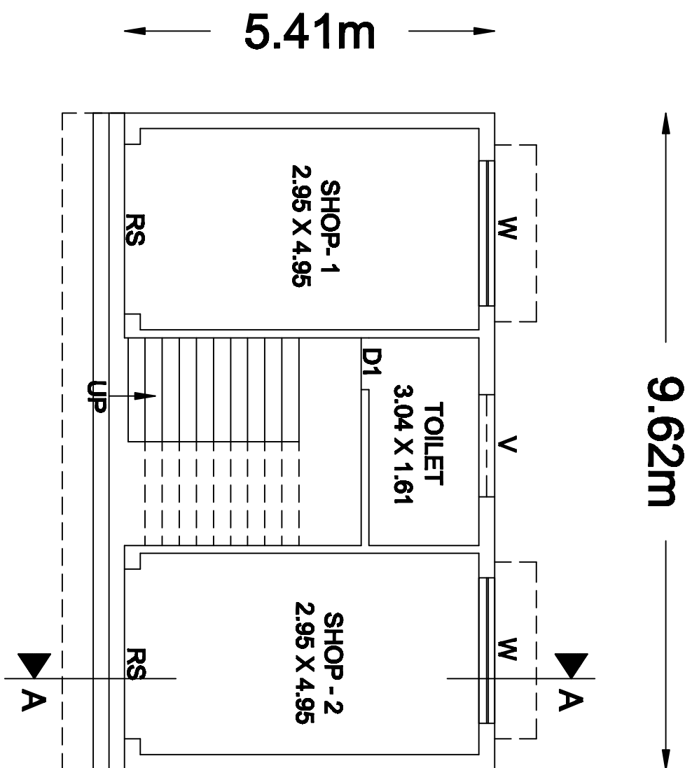
EX GROUND FLOOR PLAN
