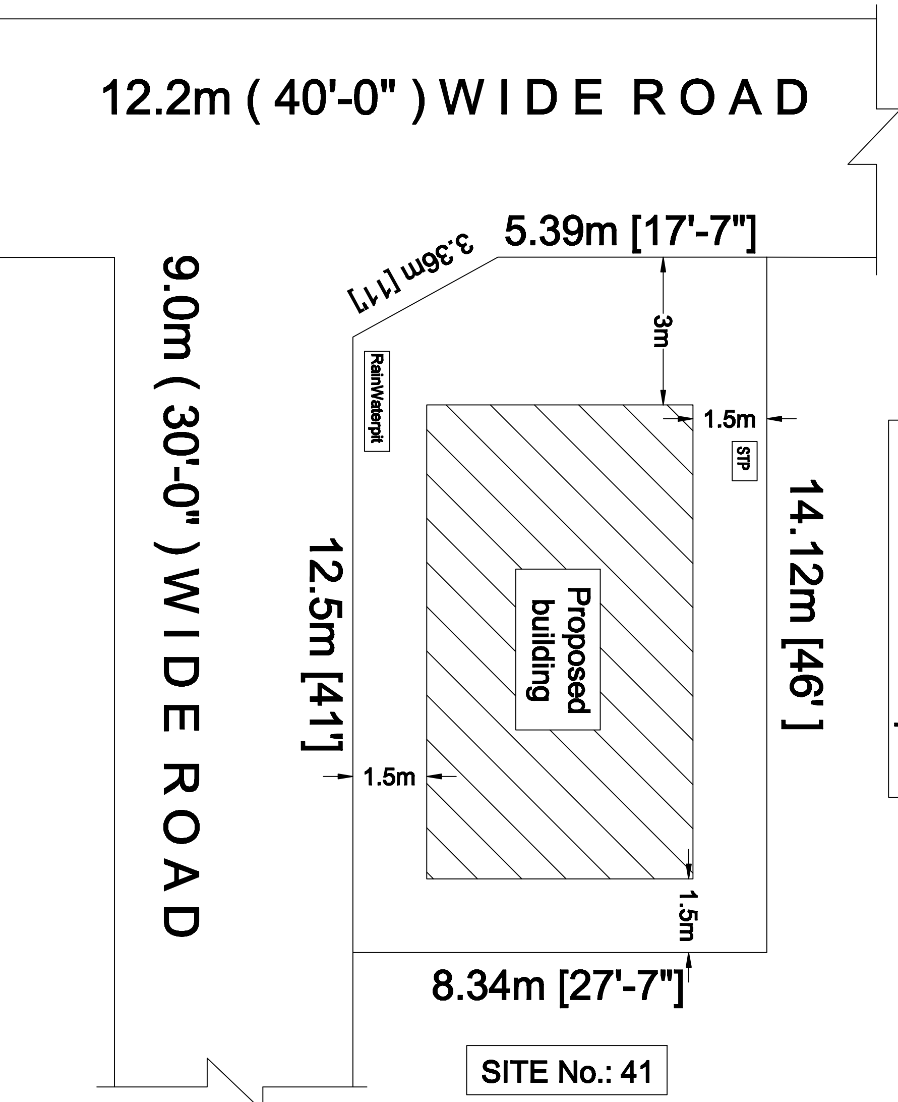
SITE PLAN
