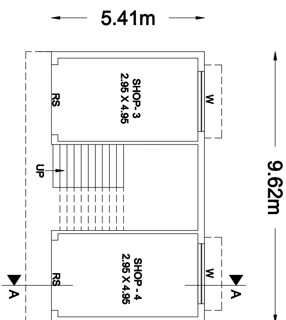
EX FIRST FLOOR PLAN
