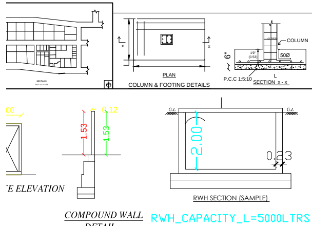
COMPOUND WALL DETAIL RWH_CAPACITY_L=5000LTRS
