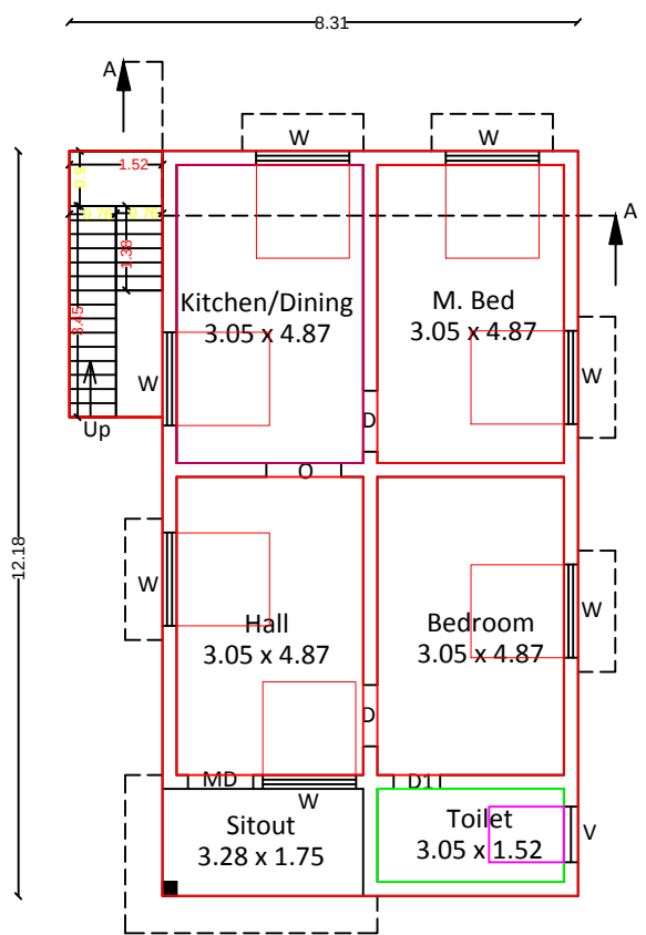
PRO.GF PLAN
