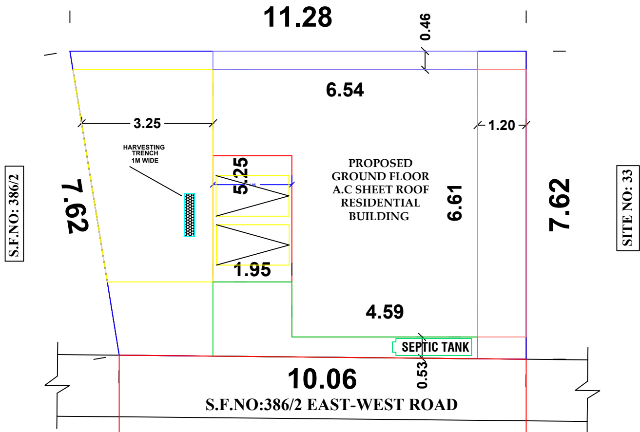
SITE PLAN
