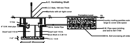
SEPTIC TANK WITH DISPERSION TRENCH ( 250 Gls., )
