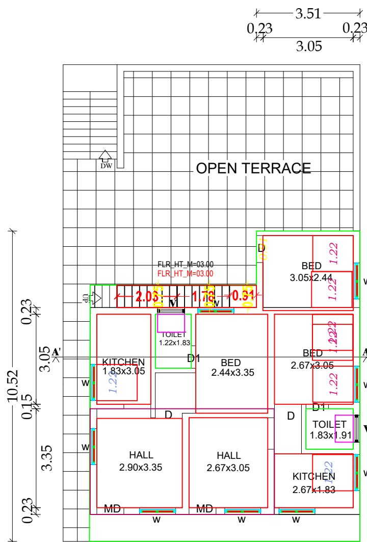
PRO. ADD. FIRST FLOOR PLAN
