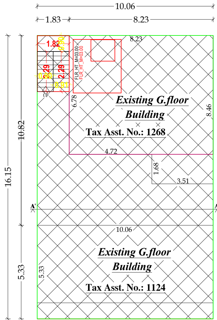
EXL. GROUND FLOOR PLAN
