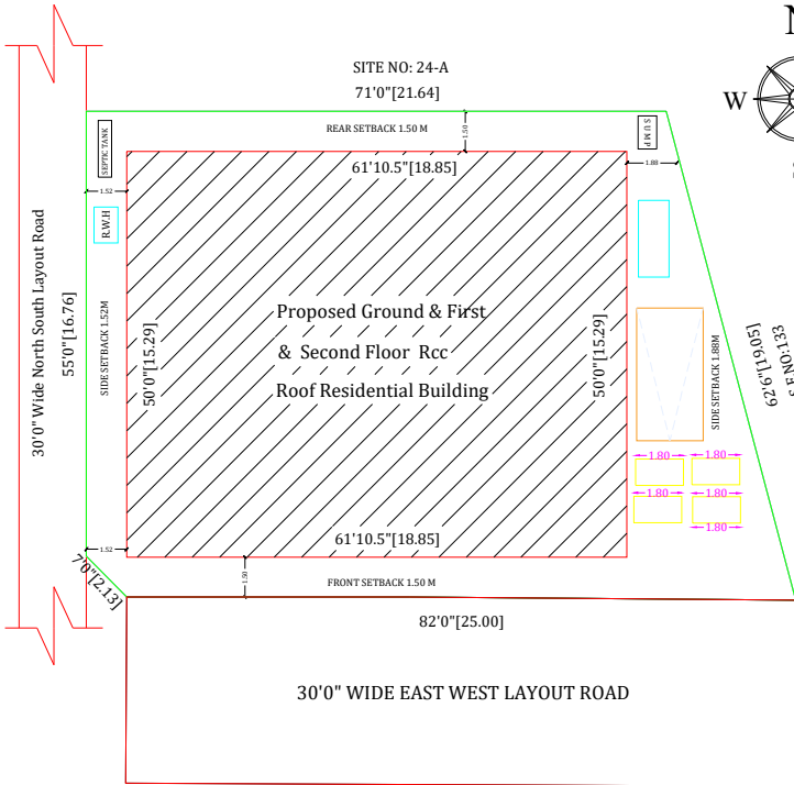
SITE PLAN
