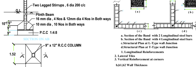
a. Section of the Band with 2 Longitudinal steel bars b. Section of the Band with 4 Longitudinal steel bars c. Structural Plan at L-Type wall Junction d. Structural Plan at T-Type wall Junction 1. Longitudinal Reinforcements 2. Lateral Tiles 3. Vertical Reinforcement at corners b.b1,b2 Wall Thickness
