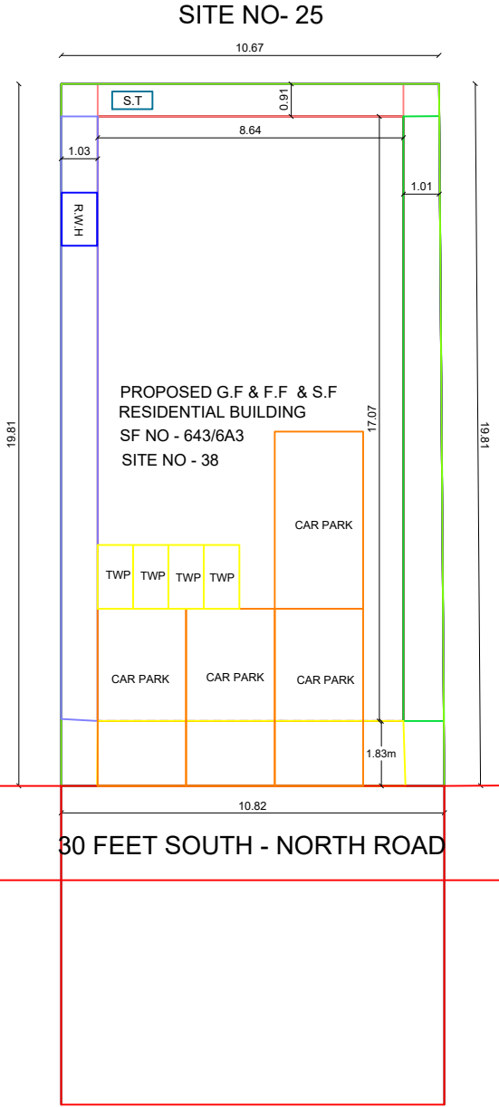
SITE PLAN
