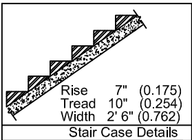
Stair Case Details
