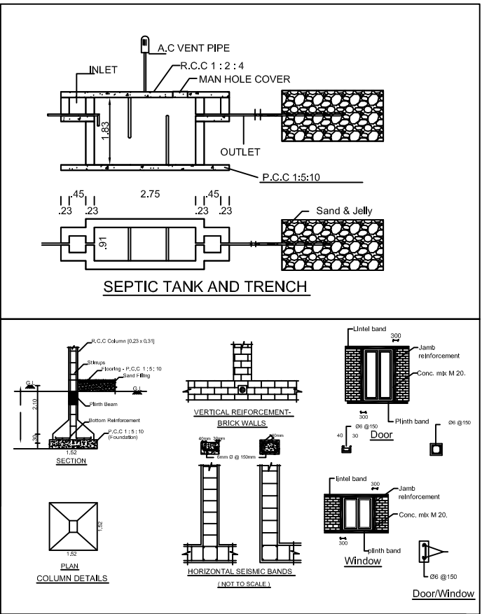
SEPTIC TANK AND TRENCH
