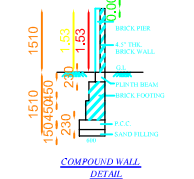
Cross Section of Rain Water Percolation Pit
