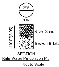
Rain Water Percolation Pit Not to Scale
