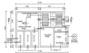
PLAN (SEWAGE TREATMENT PLANT)
