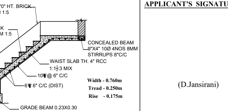
STAIRCASE DETAILS
