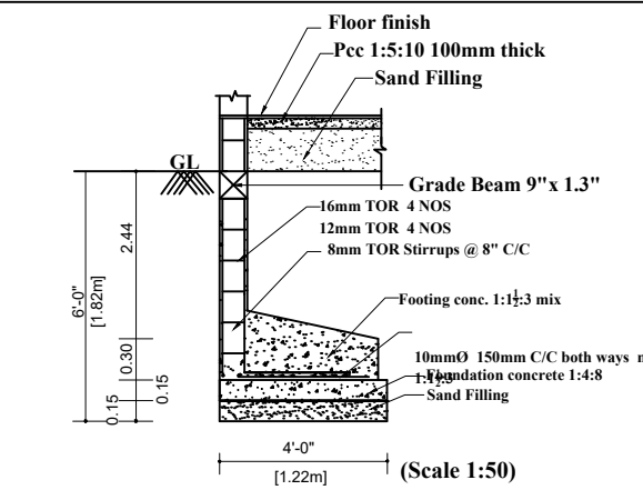
FOUNDATION DETAILS
