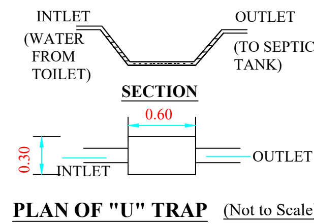
PLAN OF "U" TRAP (Not to Scale)
