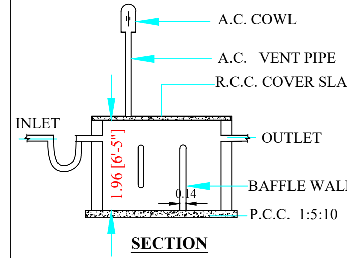
SECTION
