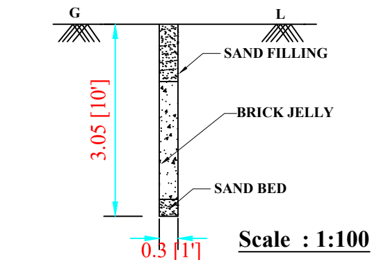
RAINWATER PERCOLATION PIT
