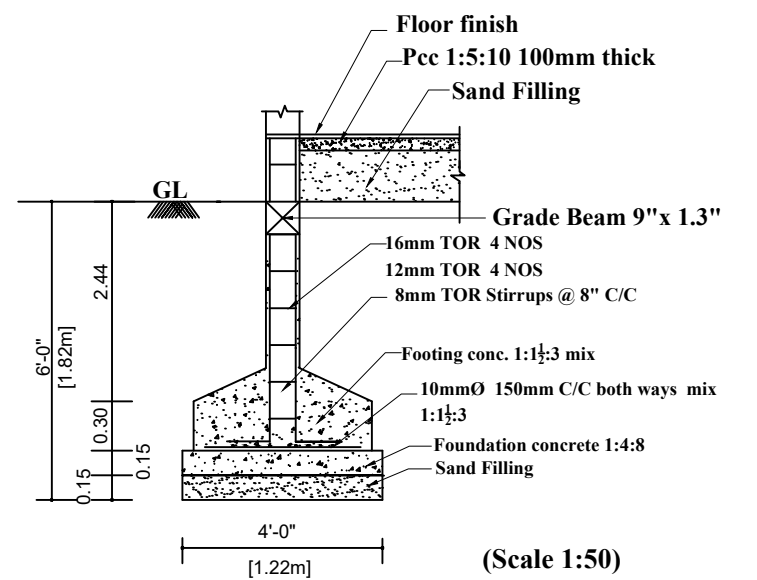
FOUNDATION DETAILS
