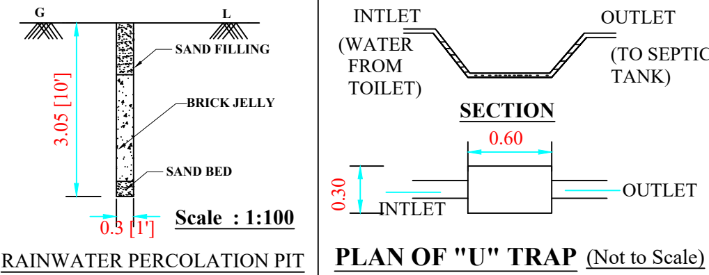
PLAN OF "U" TRAP (Not to Scale)
