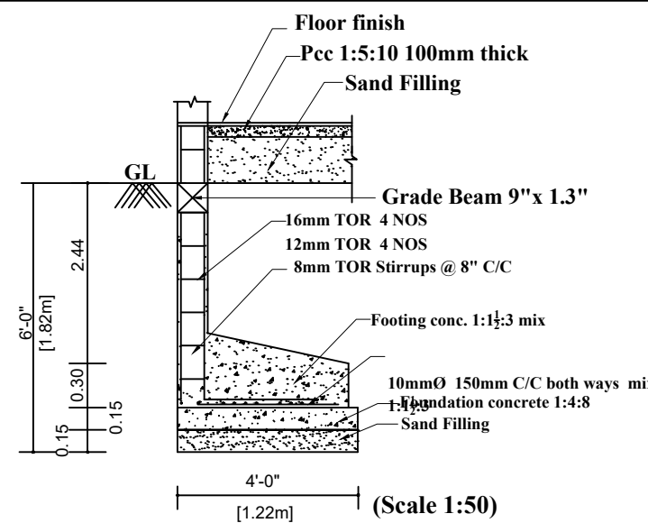
FOUNDATION DETAILS
