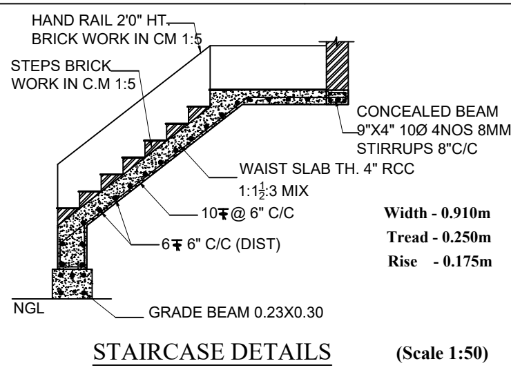
STAIRCASE DETAILS
