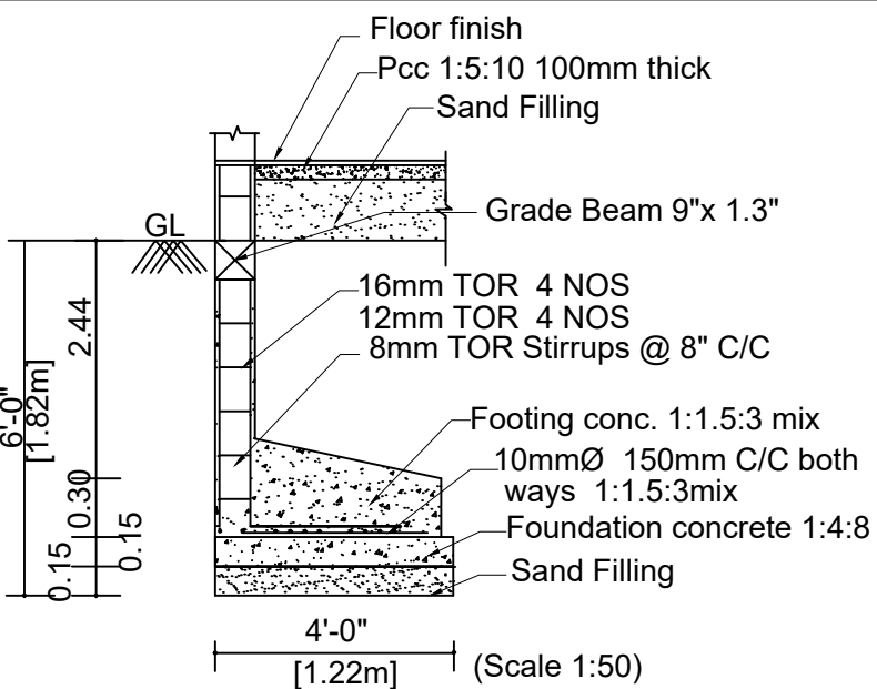
FOUNDATION DETAILS
