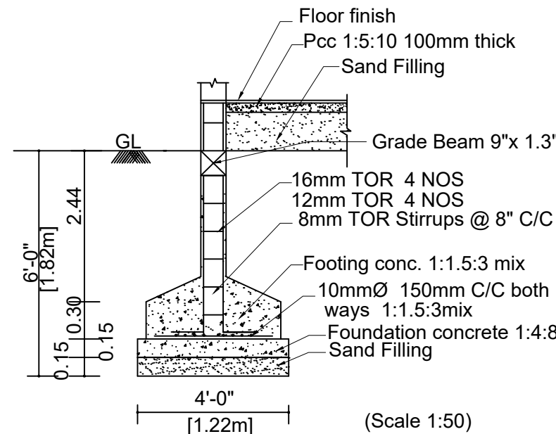
FOUNDATION DETAILS
