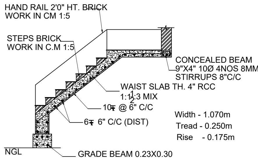
STAIRCASE DETAILS
