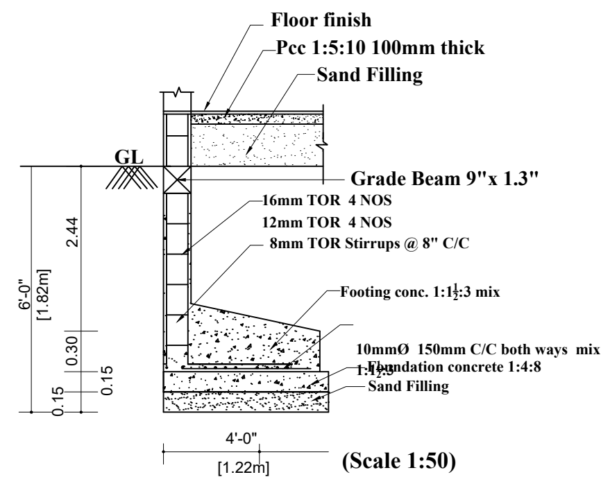
FOUNDATION DETAILS
