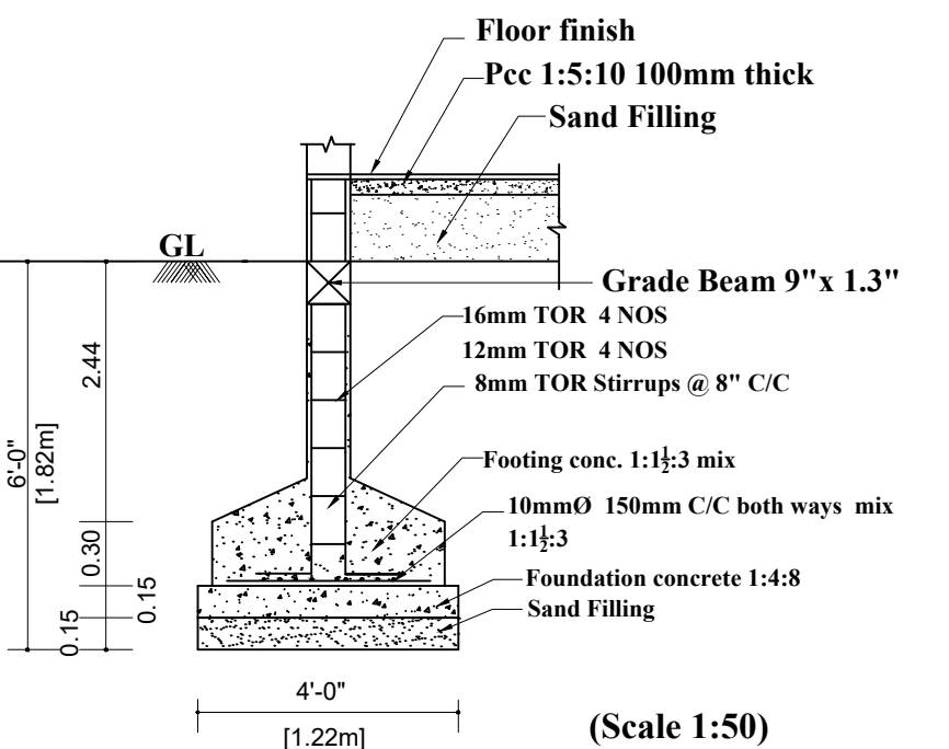
FOUNDATION DETAILS
