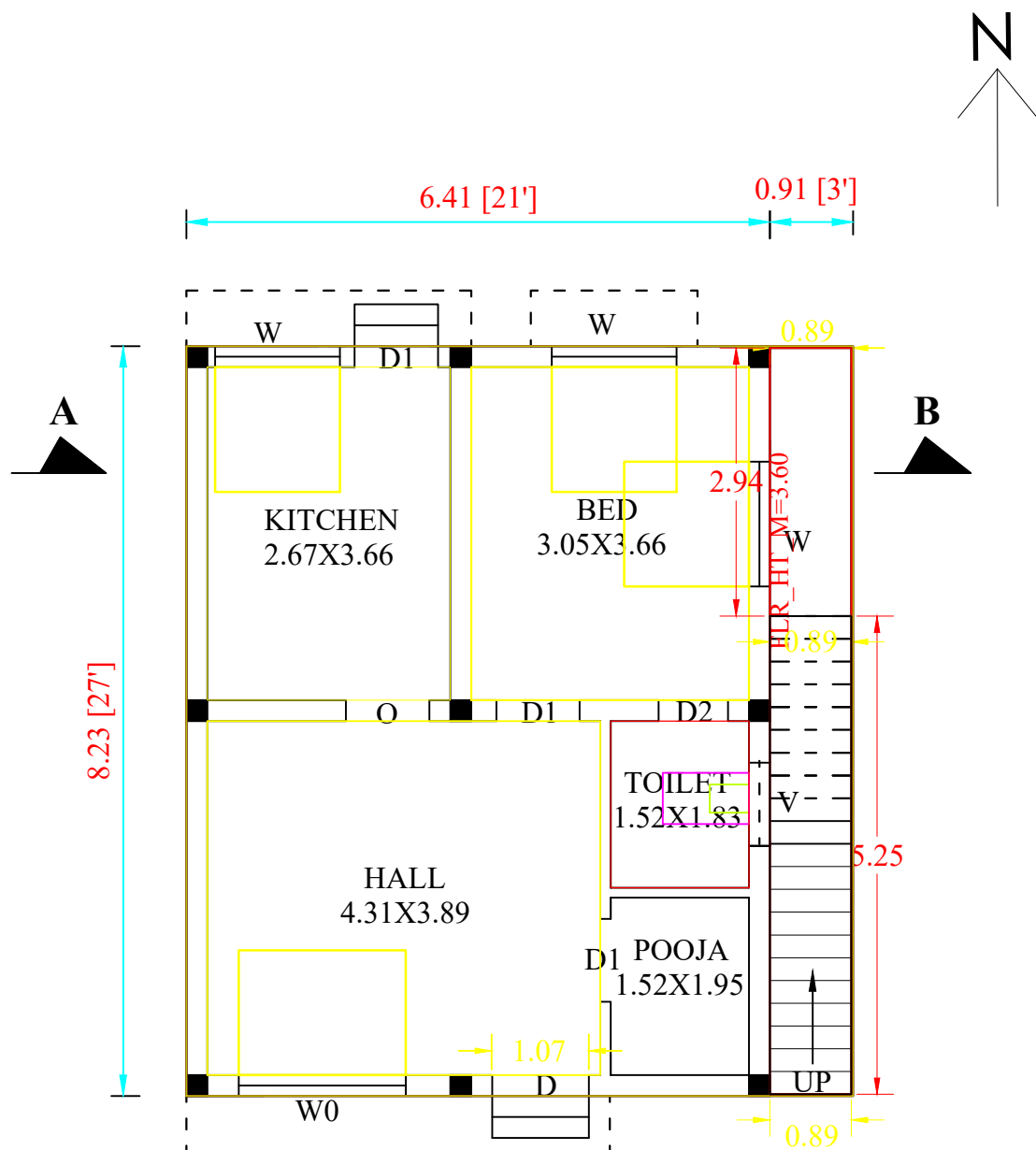
GROUND FLOOR PLAN - (SOUTH FACE)
