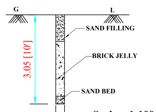
RAINWATER PERCOLATION PIT
