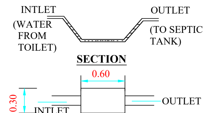
PLAN OF "U" TRAP (Not to Scale)
