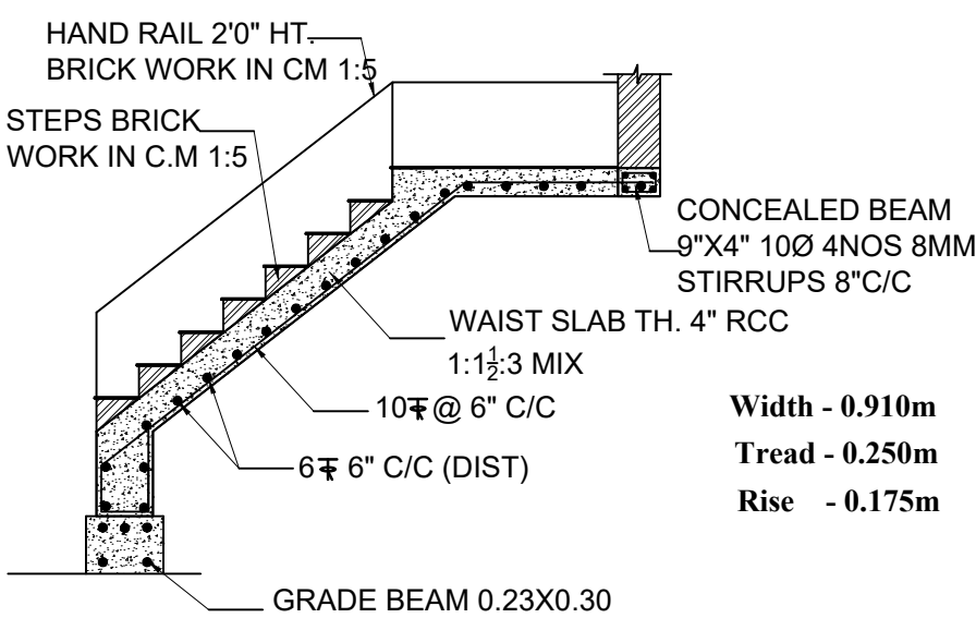
STAIRCASE DETAILS (Scale 1:50)
