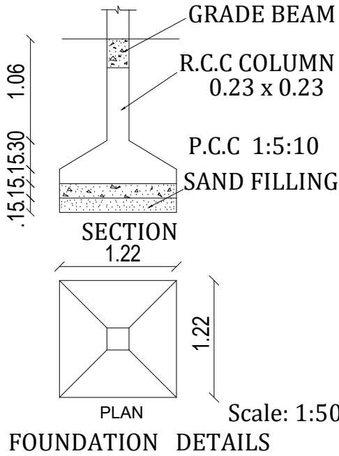
FOUNDATION DETAILS
