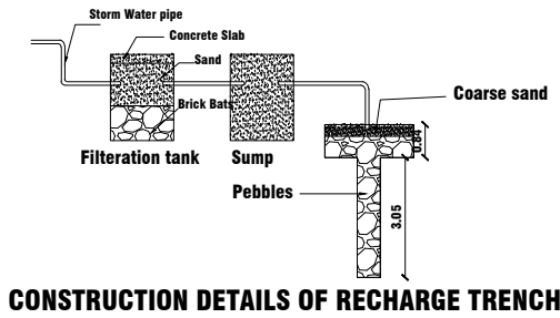
CONSTRUCTION DETAILS OF RECHARGE TRENCH
