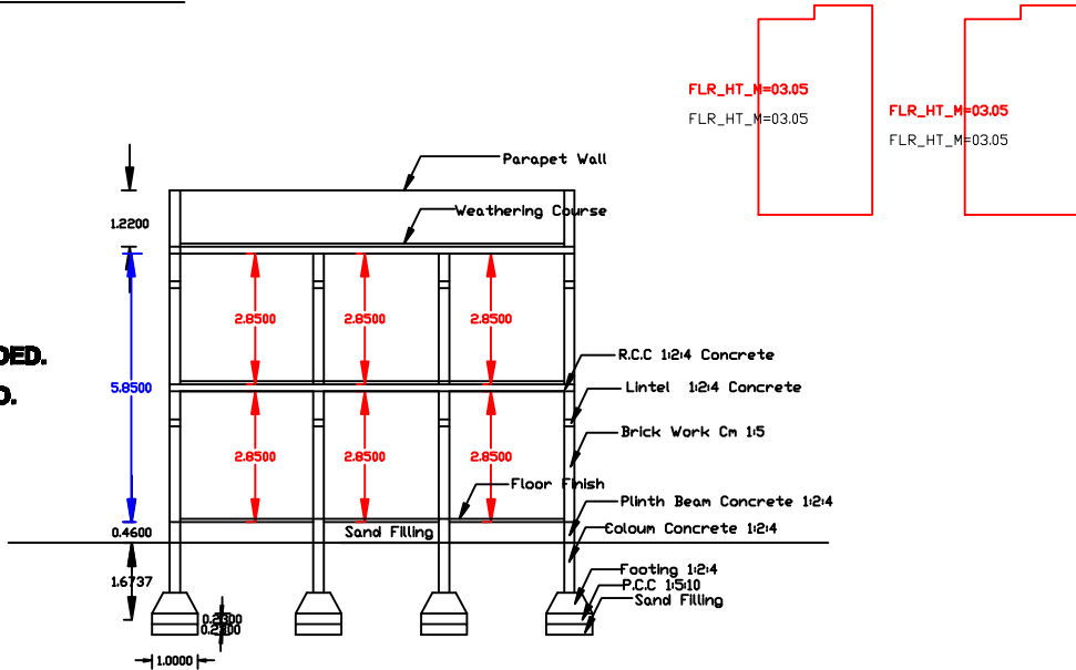
Section Section - AA
