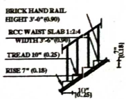
STAIRCASE DETAIL (SCALE 1:50)
