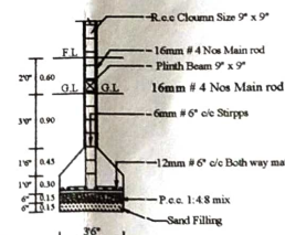
COLUMN DETAIL
