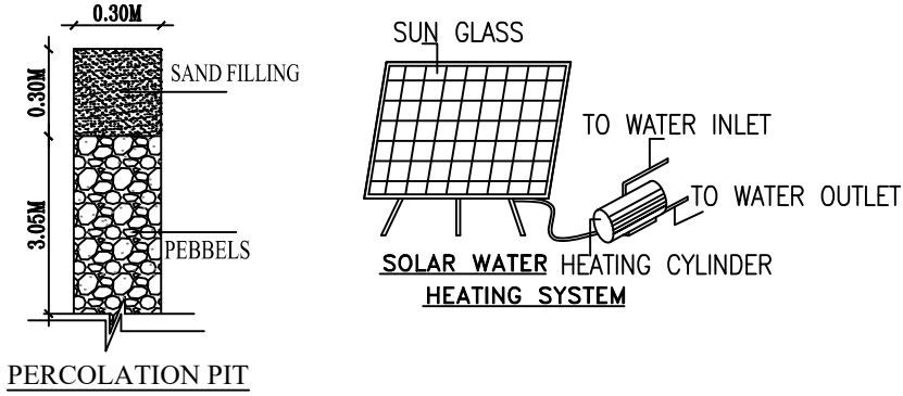
PERCOLATION PIT
