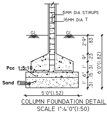
COLUMN FOUNDATION DETAIL SCALE 1"=4'0" (1:50)
