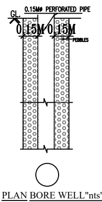
PLAN BORE WELL "nt"
