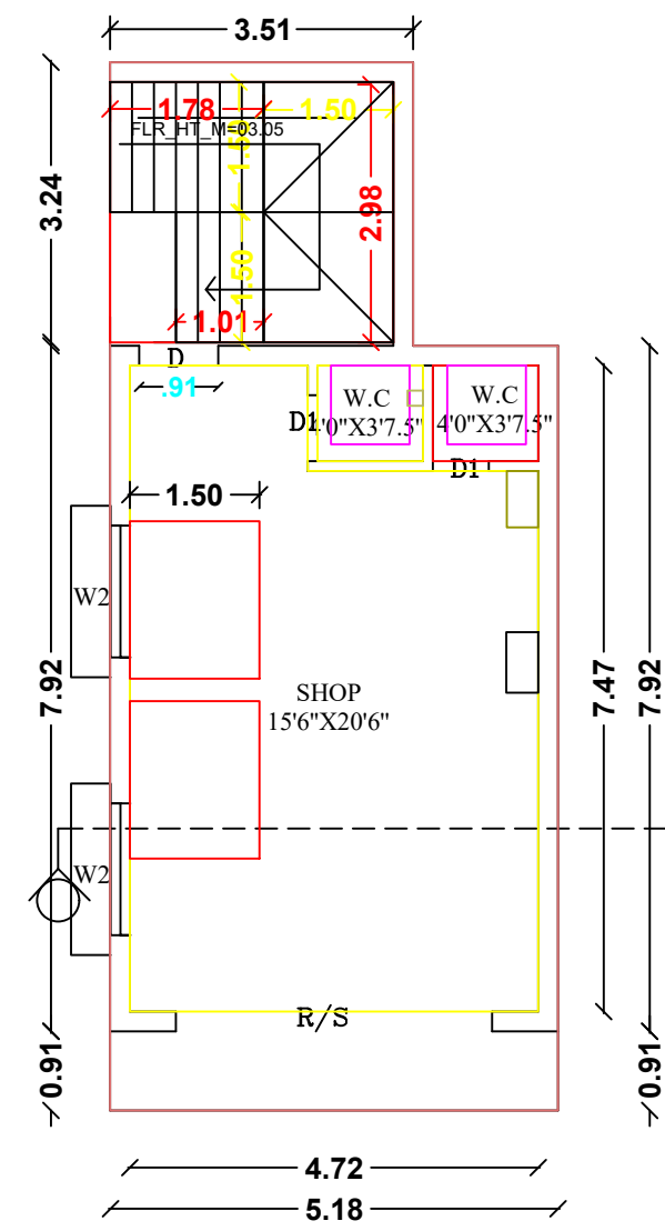
PROPOSED GROUND FLOOR PLAN (COMMERCIAL BUILDING)
