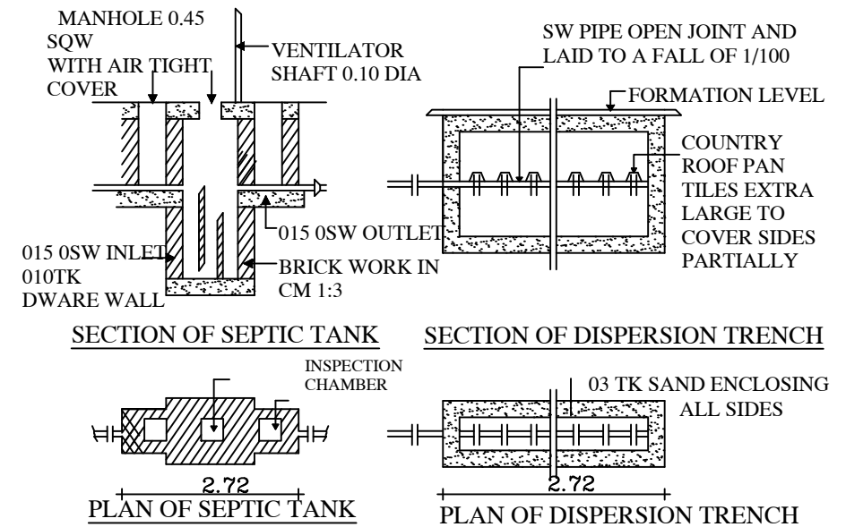
SECTION OF SEPTIC TANK SECTION OF DISPERSION TRENCH PLAN OF SEPTIC TANK PLAN OF DISPERSION TRENCH
