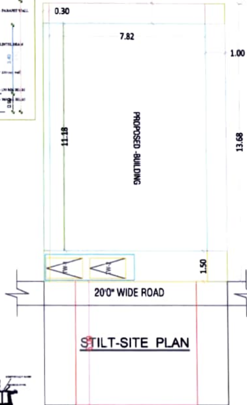
STILT-SITE PLAN
