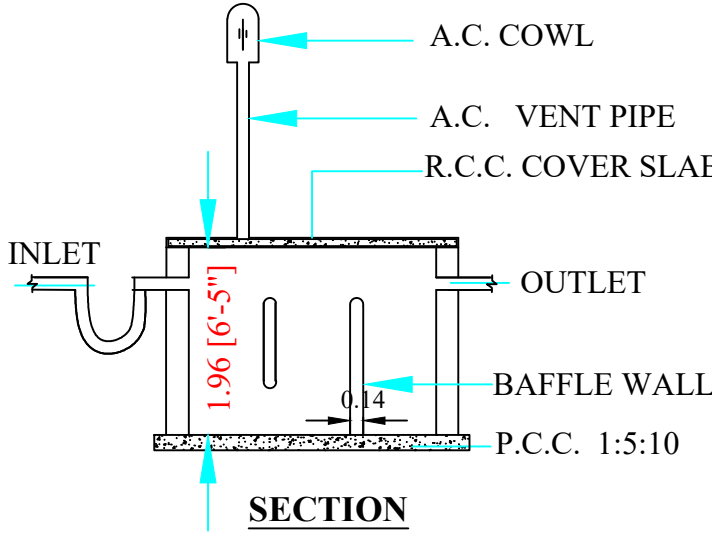
SECTION
