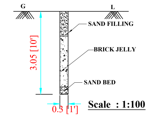
RAINWATER PERCOLATION PIT
