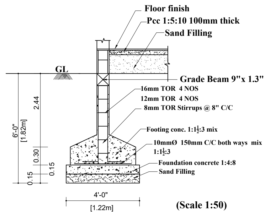
FOUNDATION DETAILS
