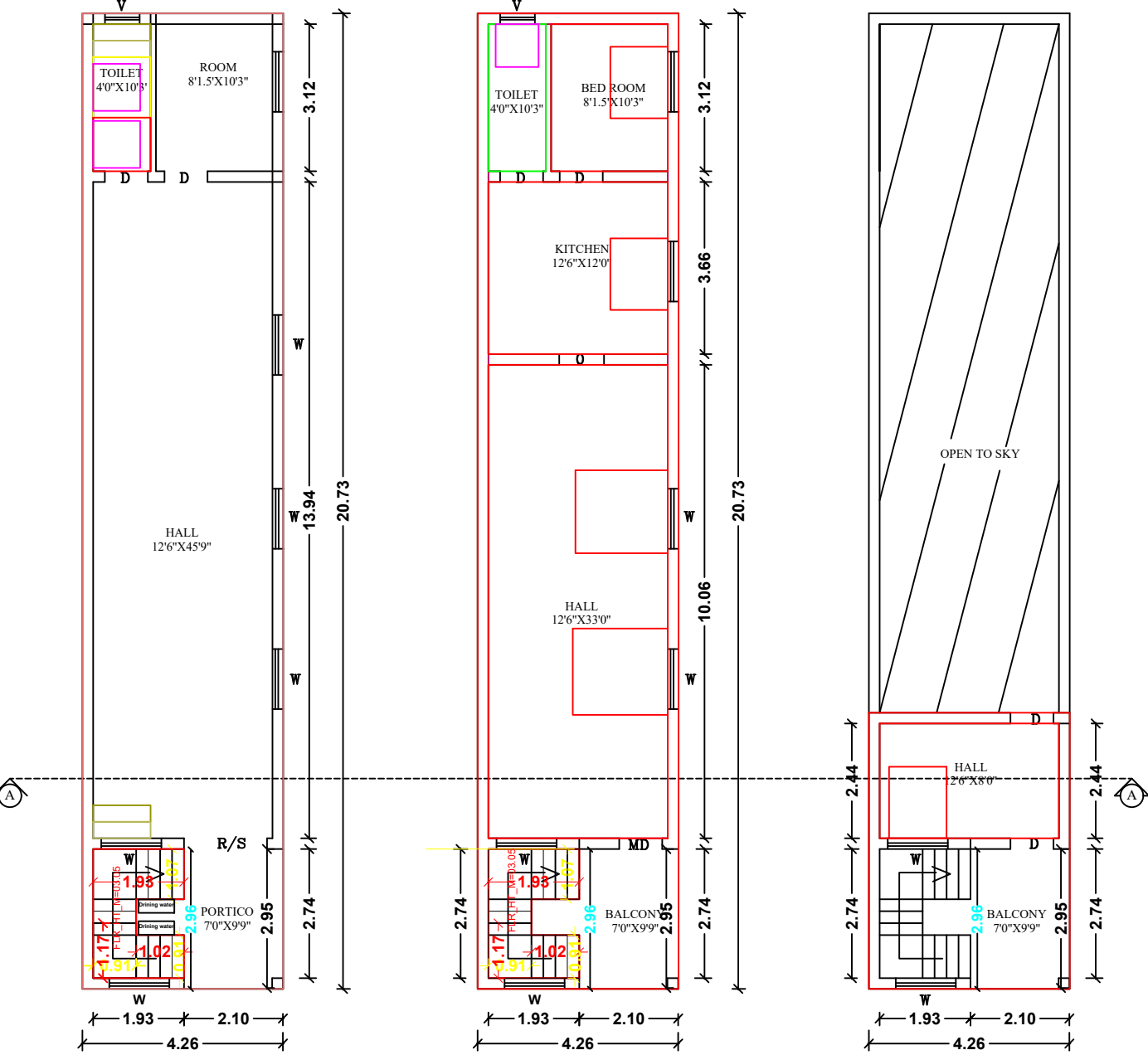
EXISTING GROUND FLOOR PLAN PROPOSED FIRST FLOOR PLAN PROPOSED SECOND FLOOR PLAN
