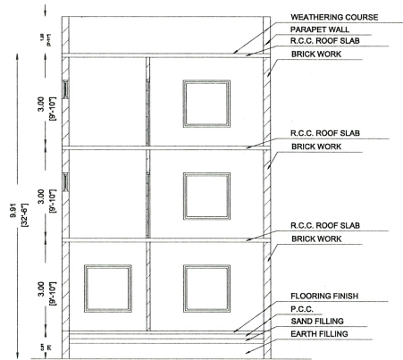
SECTION ON XX
