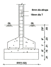
COLUMN FOUNDATION DETAIL
