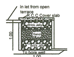
RAIN WATER HARVESTING
