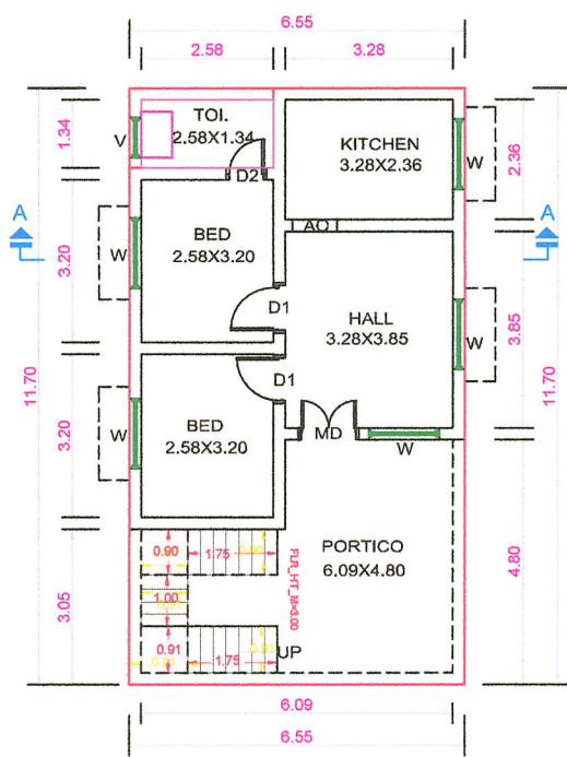
EXI.GROUND FLOOR PLAN
